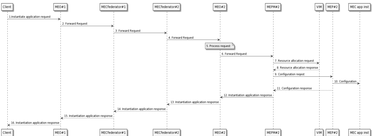
Figure 5.2.2.5.3-1: Application instantiation flow in MEC federation
