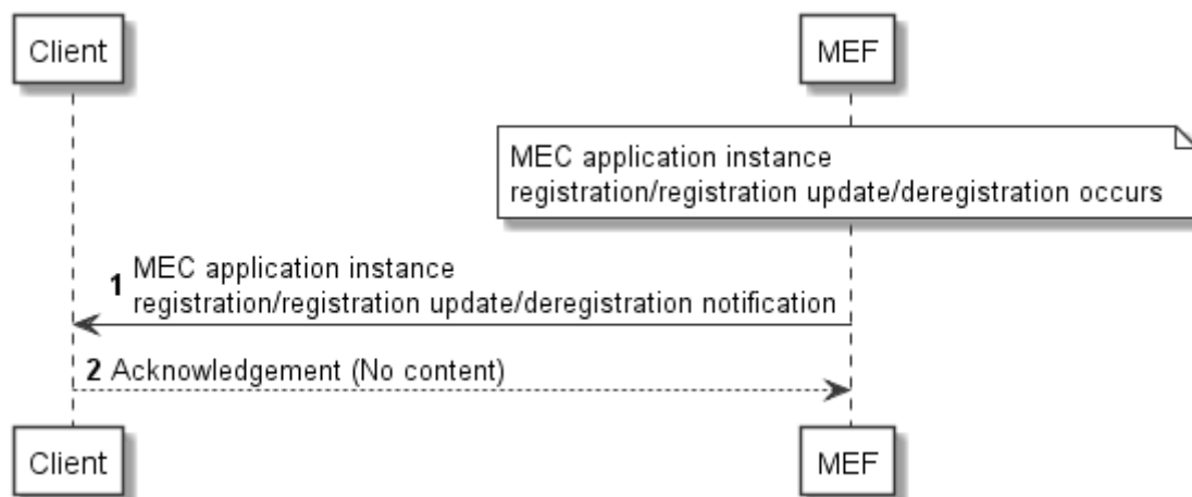
Figure 5.2.X3-1: Information flow of receiving MEC application instance registration/registration update/deregistration notification
