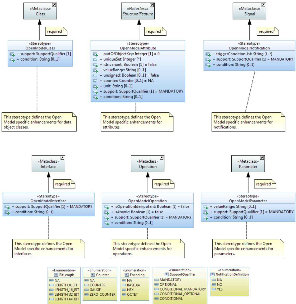
Figure 6.2-1: Required "Stereotypes"
