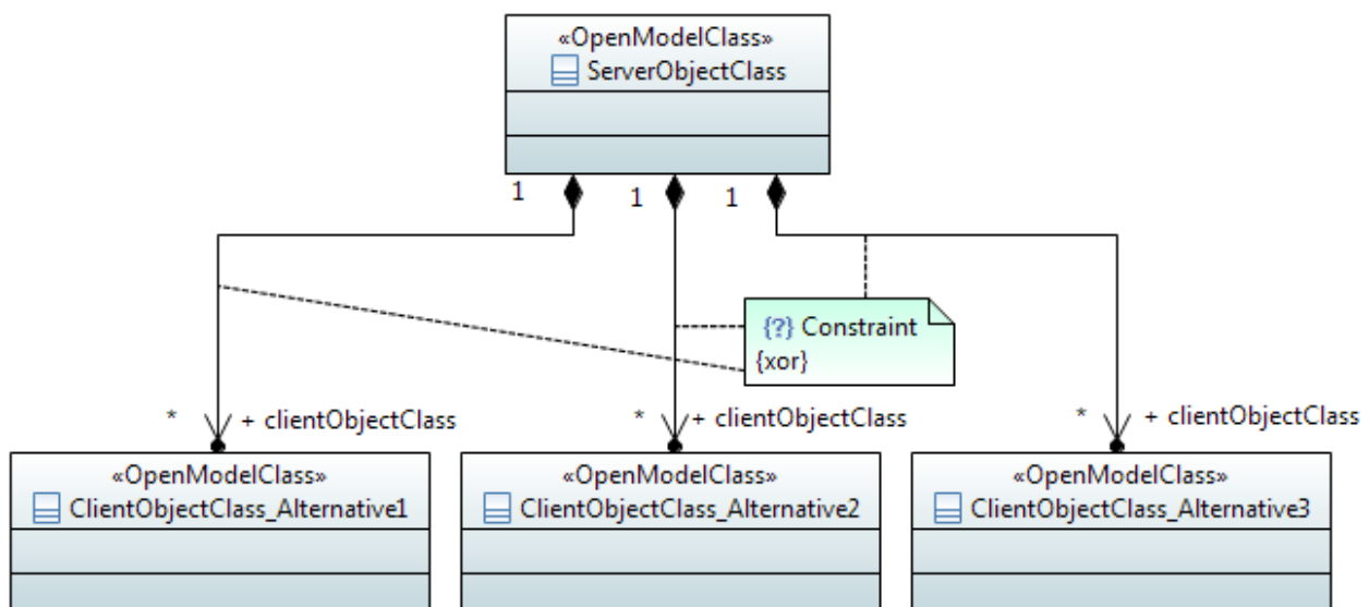
Figure 7.2.1.2-1: {xor} notation
