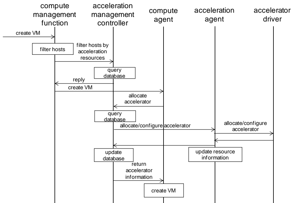
Figure B.2.2.1-1: Acceleration resource allocation
