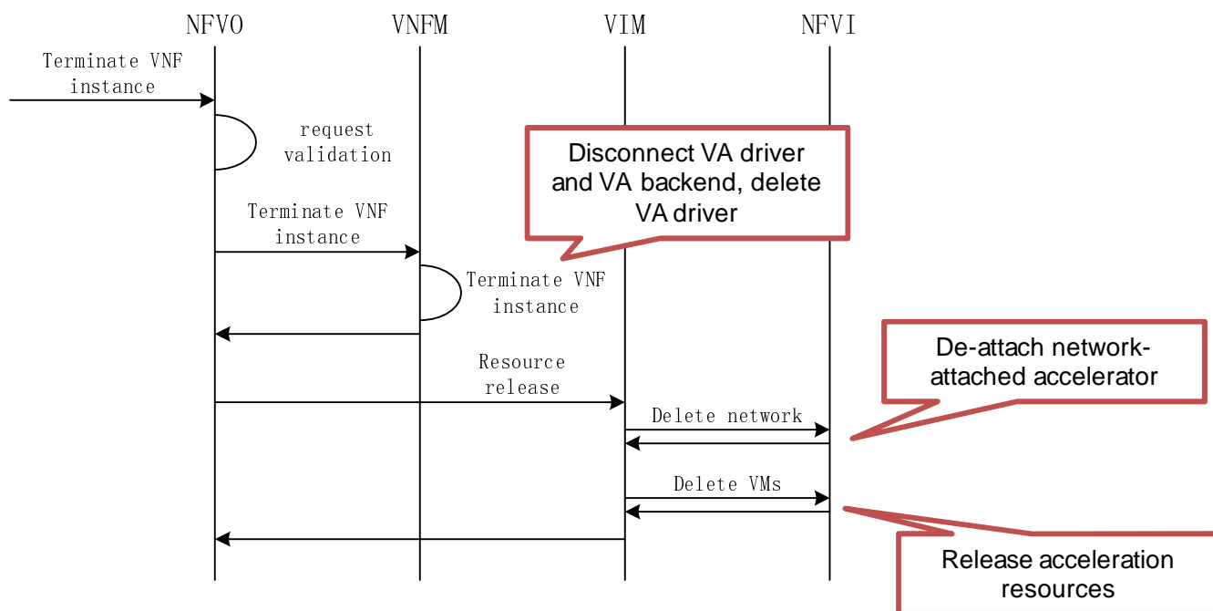
Figure A.3-1: Acceleration resource release in indirect mode
