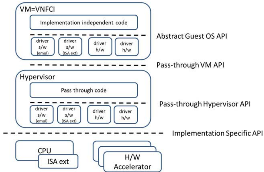
Figure 4-2: NFV acceleration abstraction layer implemented within VNF as an integrated model
