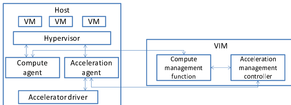
Figure B.2.1-1: Acceleration management architecture example
