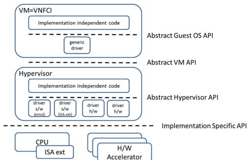
Figure 4-1: NFV acceleration abstraction layer implemented within hypervisor as a disaggregated model
