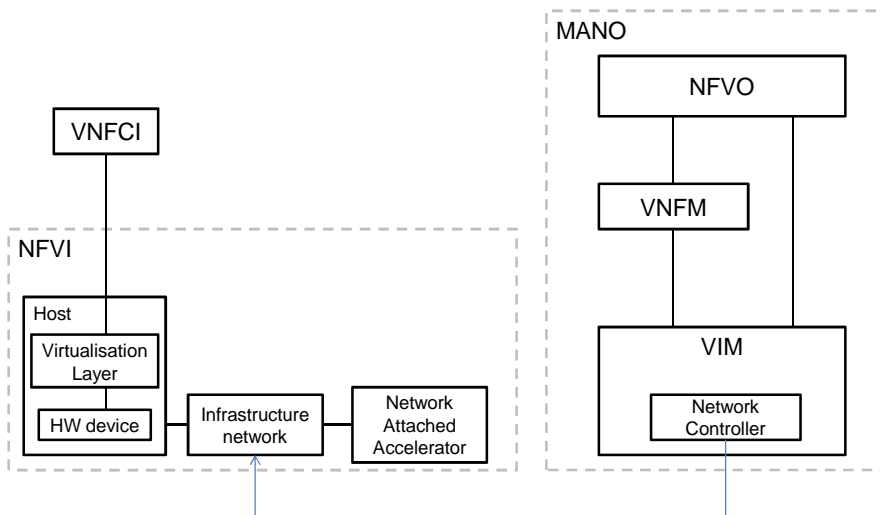
Figure 5.2-1: VNF and accelerator interconnection
