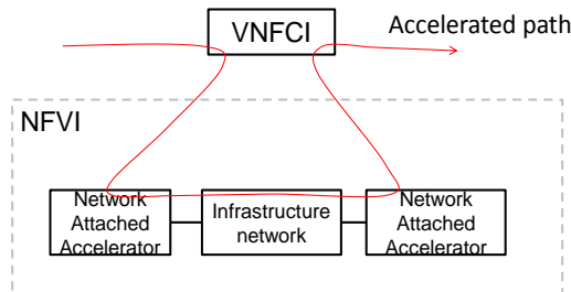
Figure 5.2-2: Accelerator chaining
