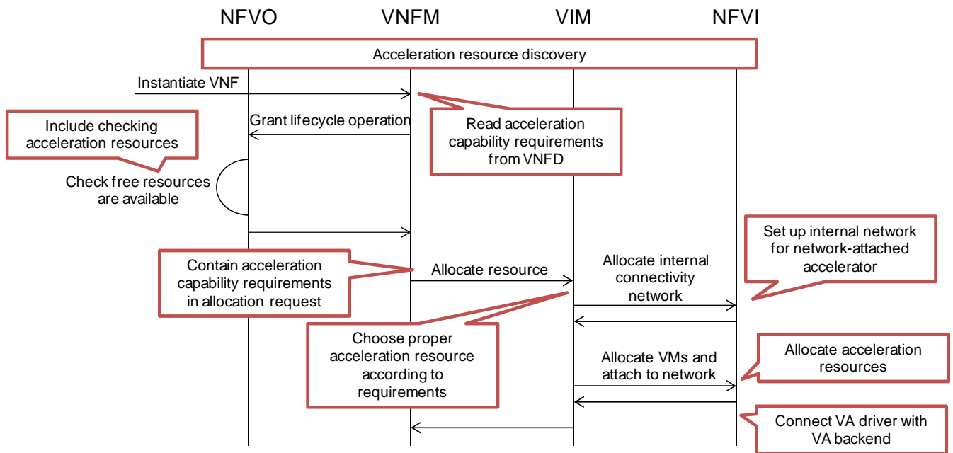
Figure A.2-2: Acceleration resource allocation in direct mode
