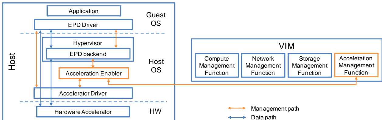
Figure 4.2.1-1: Acceleration resource management architecture
