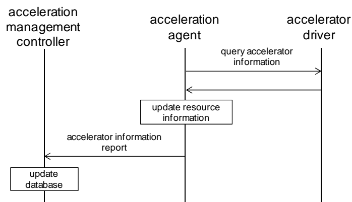
Figure B.2.2.2-1: Acceleration resource discovery
