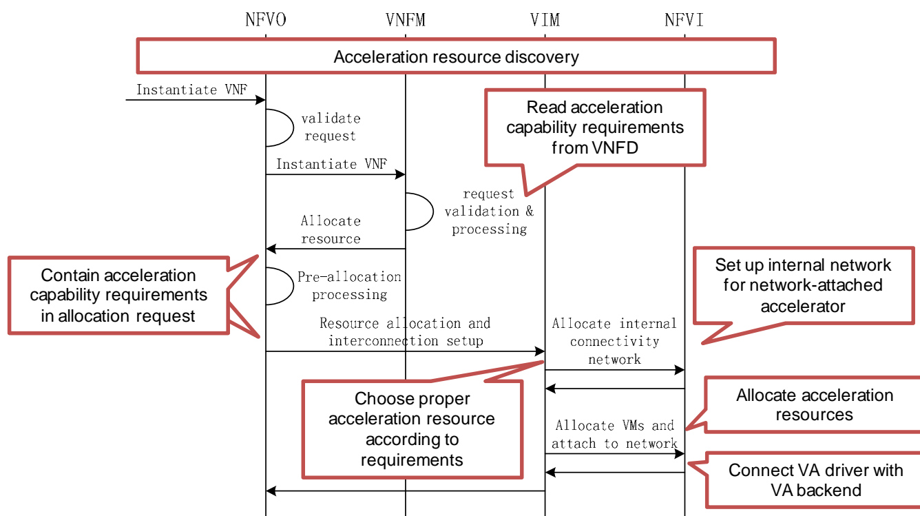
Figure A.2-1: Acceleration resource allocation in indirect mode
