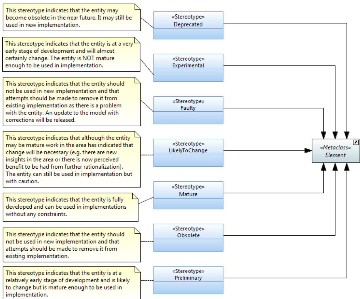
Figure 6.3.1-1: Lifecycle "Stereotypes"
