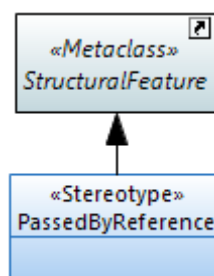
Figure 5.2.3-2: "PassedByReference" Stereotype
