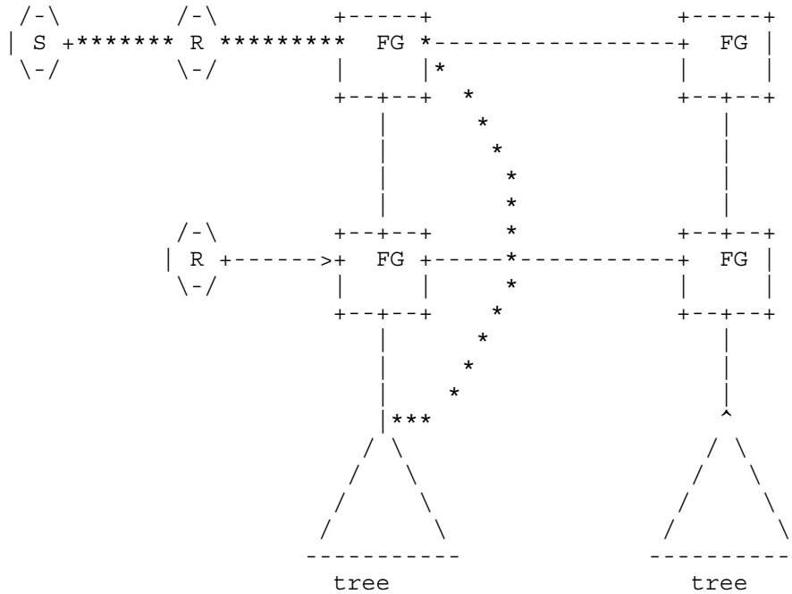
Architecture diagram, showing seekers (S), resolvers (R), forest guides (FG) and trees. The star (*) line indicates the flow of the query and responses in recursive mode.
