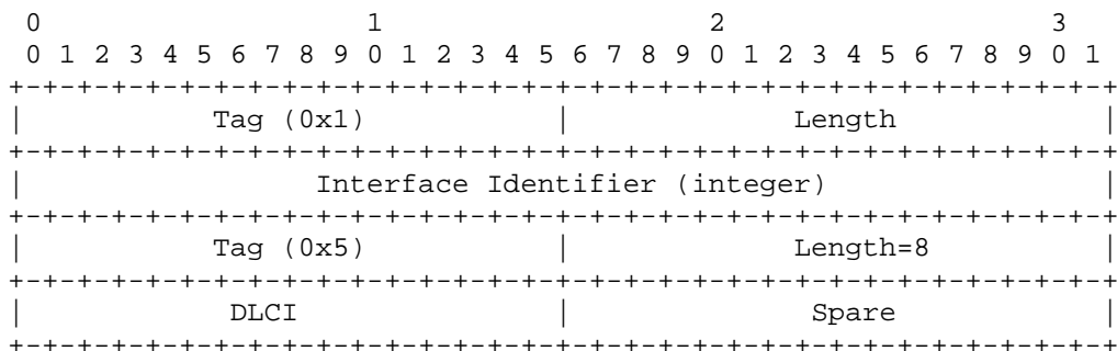
Figure 3 IUA Message Header (Integer-based Interface Identifier)
