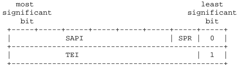
Figure 6 DLCI Format
