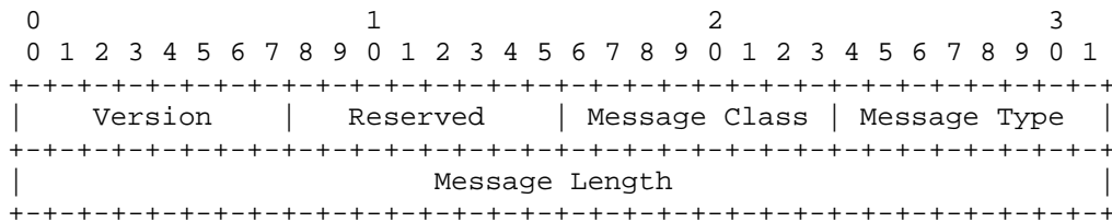
Figure 2 Common Header Format
