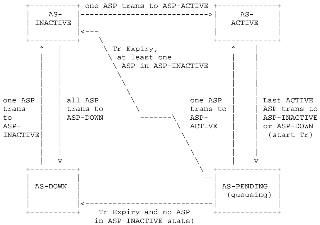
Figure 7: AS State Transition Diagram
