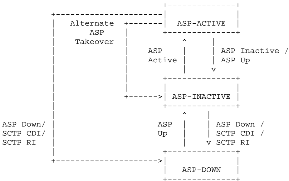
Figure 6 ASP State Transition Diagram
