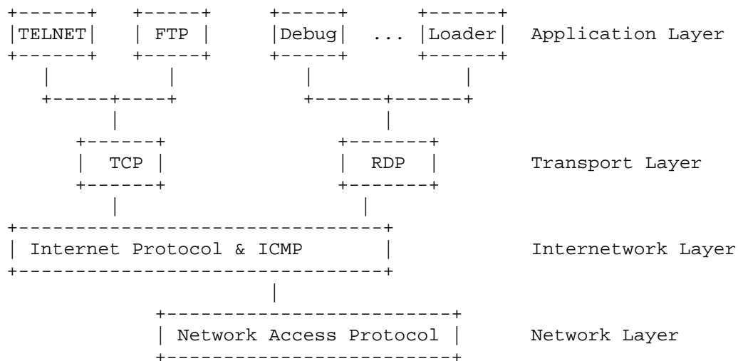
Relation to Other Protocols Figure 1
