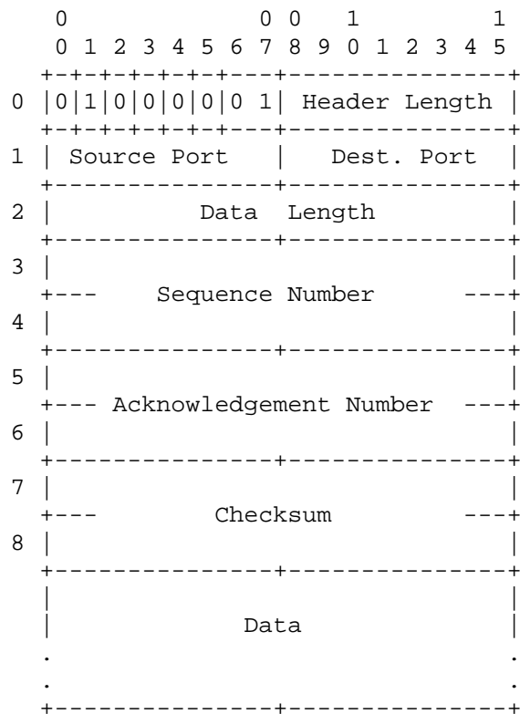
ACK Segment Format Figure 7
