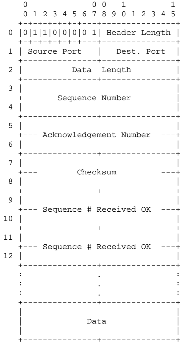
EACK Segment Format Figure 8
