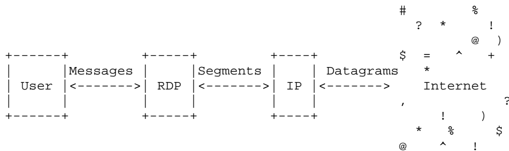
Form of Data Exchange Between Layers Figure 2
