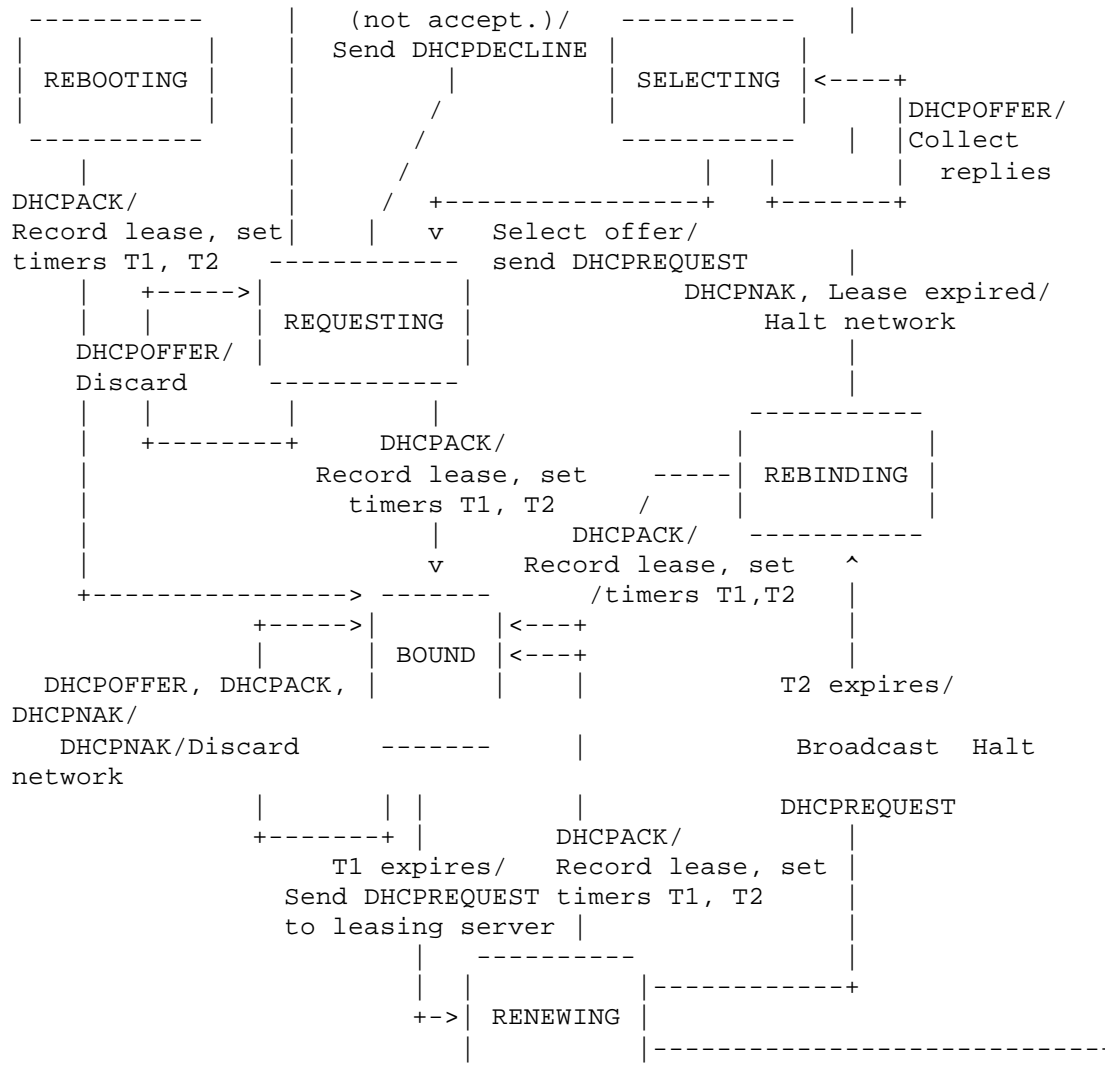
Figure 5: State-transition diagram for DHCP clients
