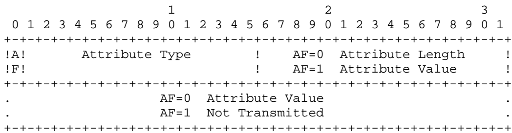
Figure 4: Data Attributes
