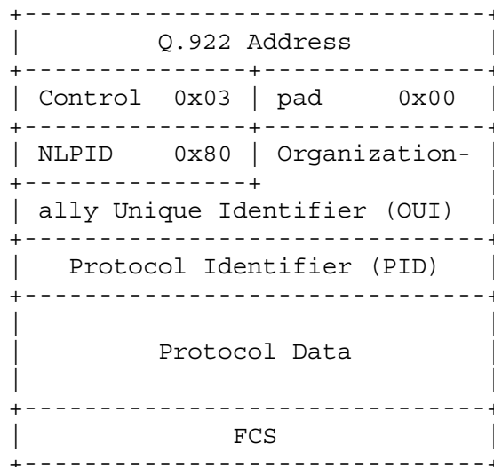
Format of Routed Frames with a SNAP Header
