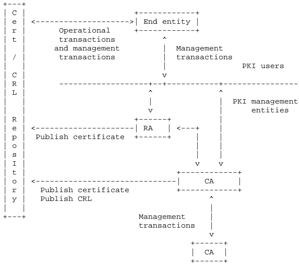
Figure 1 - PKI Entities
