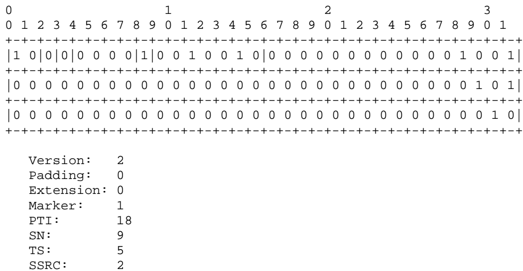
Figure 4: RTP Header for Media Packet Y
