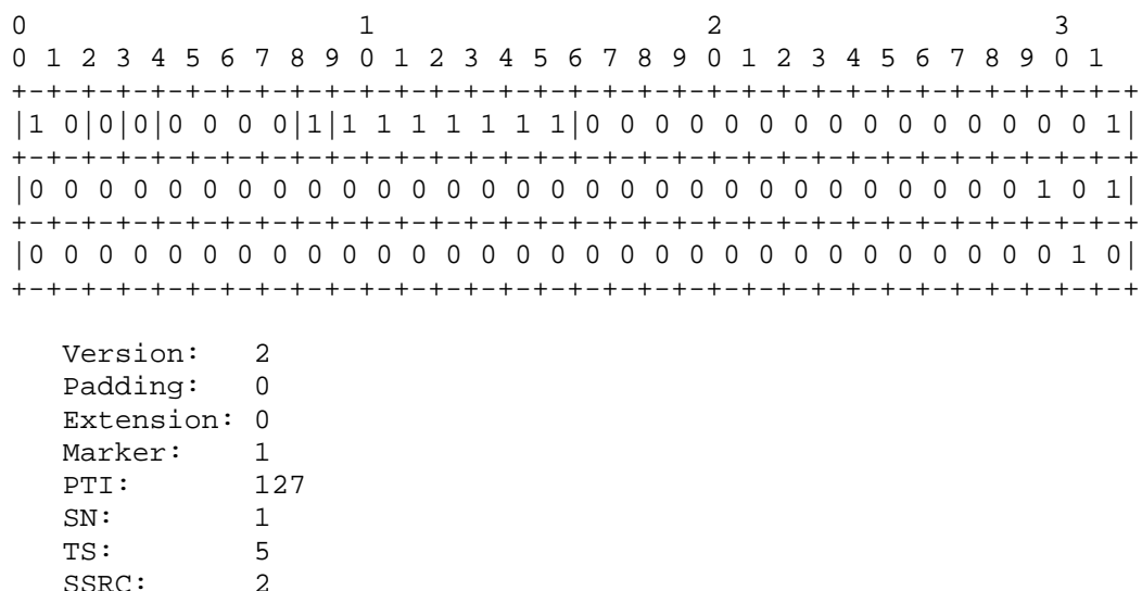
Figure 5: RTP Header of FEC for Packets X and Y
