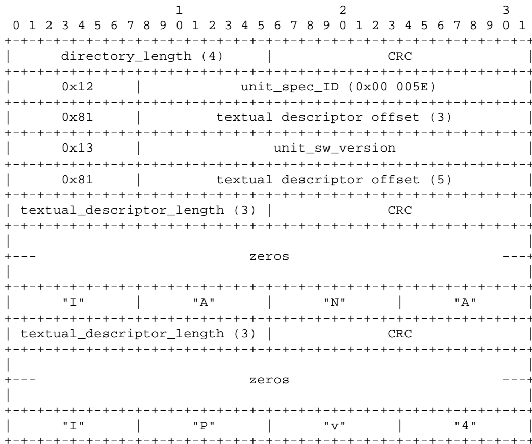
Figure 9 - Sample unit directory and textual descriptors
