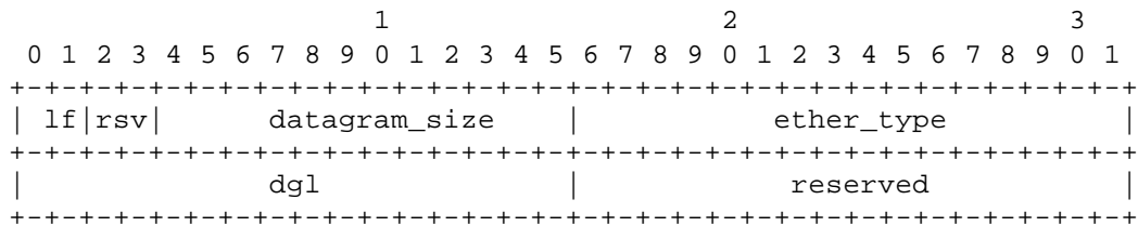
Figure 3 - First fragment encapsulation header format
