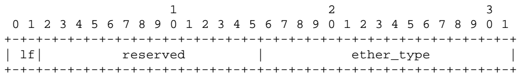
Figure 2 - Unfragmented encapsulation header format
