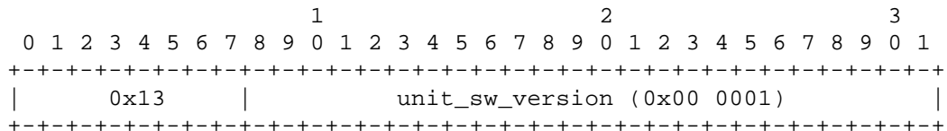
Figure 7 - Unit_SW_Version entry format
