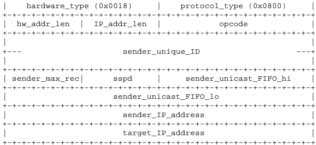
Figure 5 - 1394 ARP request/response format
