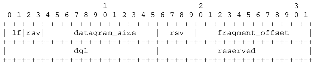
Figure 4 - Subsequent fragment(s) encapsulation header format
