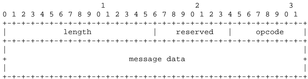
Figure 10 - MCAP message format
