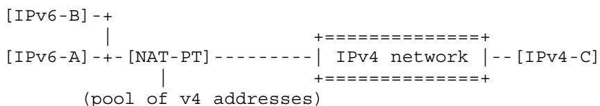
Figure 1: IPv6 to IPv4 communication
