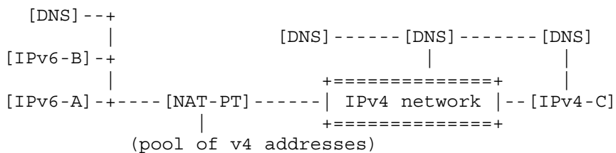
Figure 2: IPv4 to IPv6 communication Node IPv6-A has an IPv6 address -> FEDC:BA98::7654:3210 Node IPv6-B has an IPv6 address -> FEDC:BA98::7654:3211 Node IPv4-C has an IPv4 address -> 132.146.243.30
