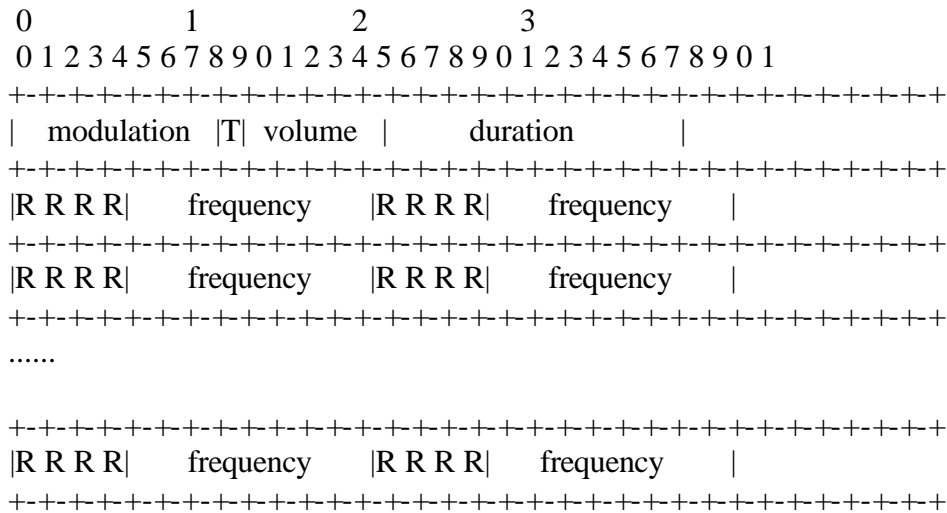
Figure 3: Payload format for tones
