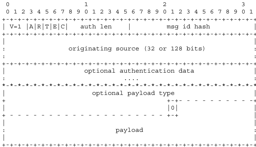
Figure 1: Packet format
