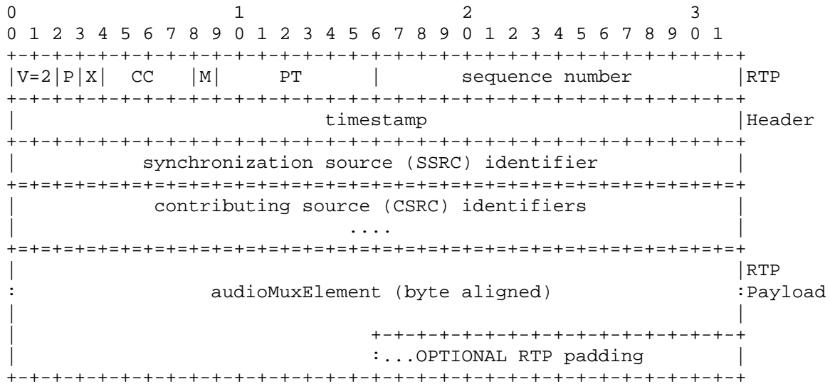
Figure 4 - An RTP packet for MPEG-4 Audio
