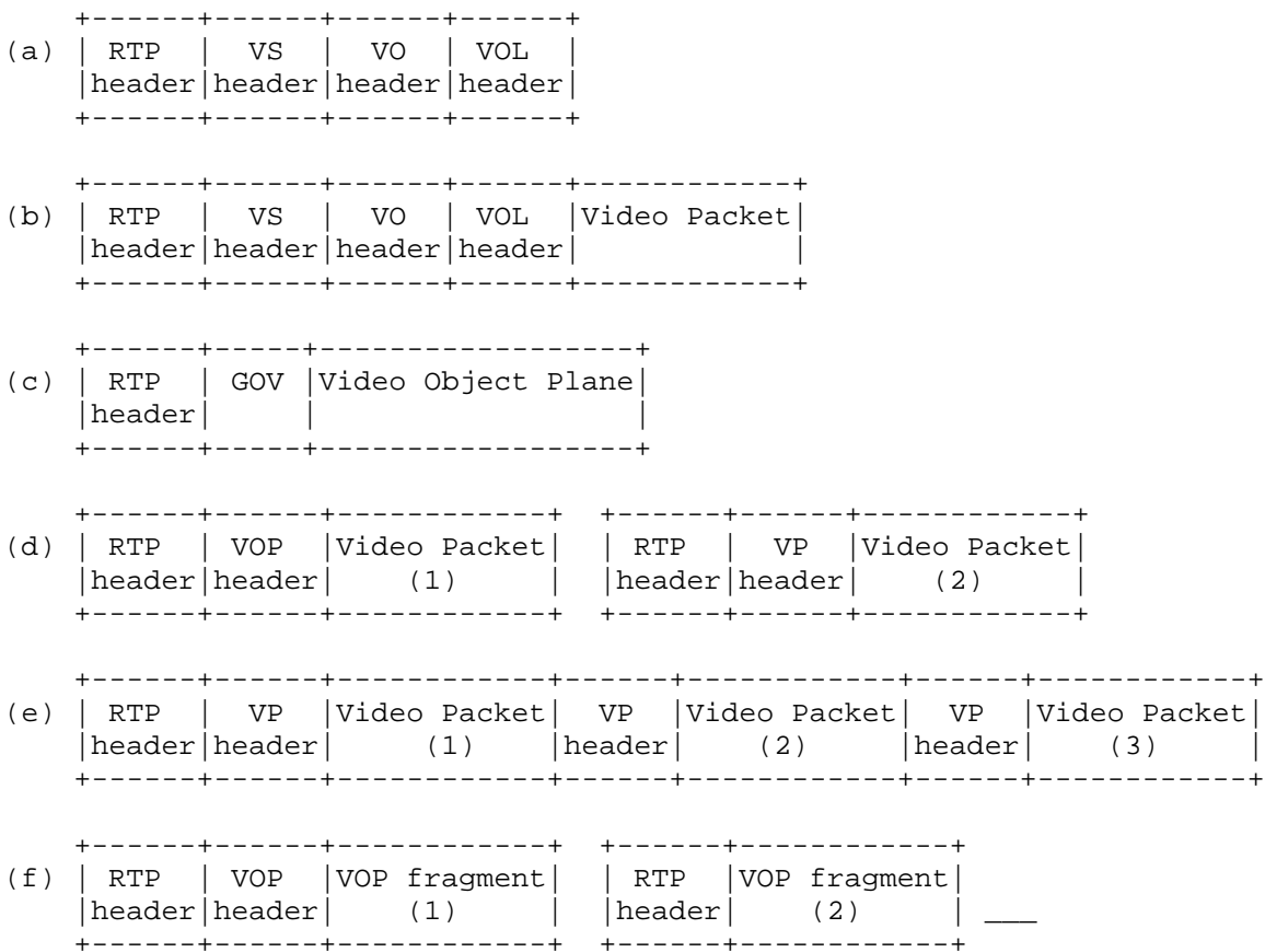
Figure 2 - Examples of RTP packetized MPEG-4 Visual bitstream
