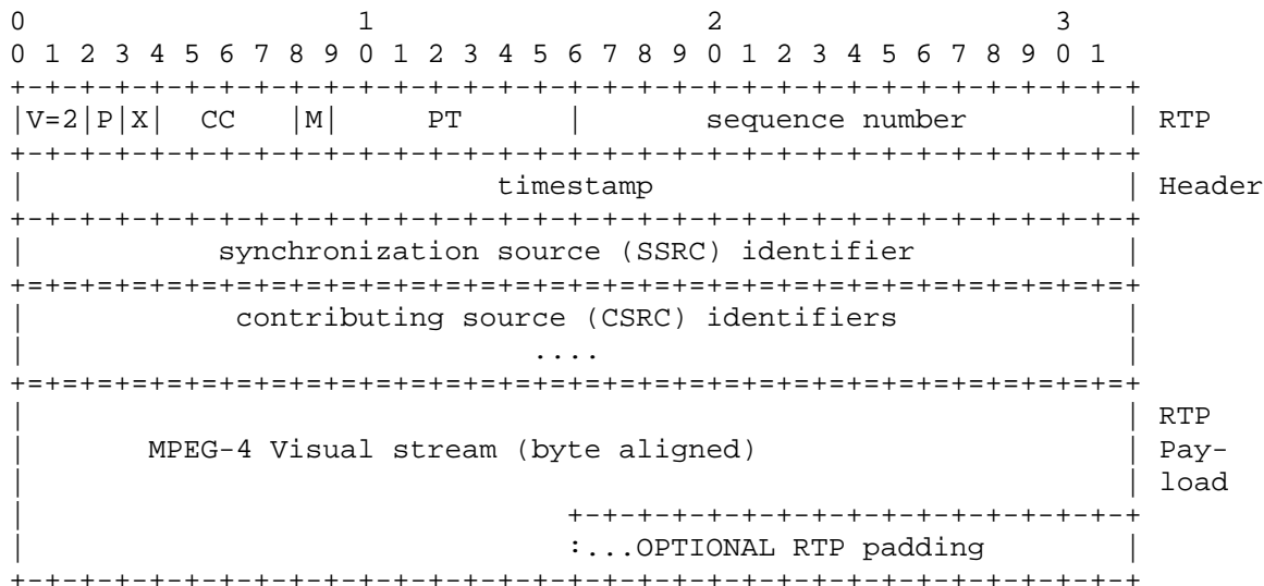
Figure 1 - An RTP packet for MPEG-4 Visual stream
