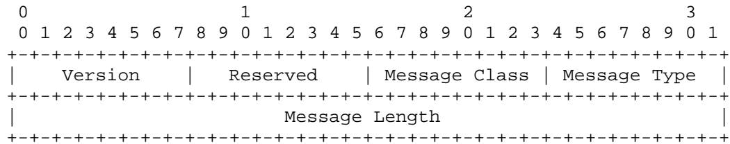
Figure 3 Common Header Format
