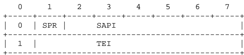
Figure 6 DLCI Format
