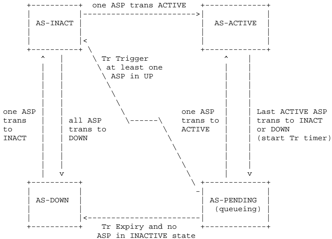
Figure 8 AS State Transition Diagram
