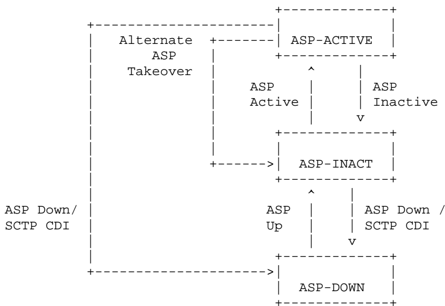
Figure 7 ASP State Transition Diagram
