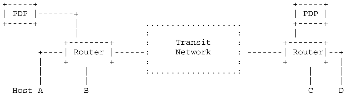
Figure 1: User and Application Authentication using AUTH_DATA PE
