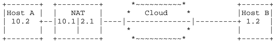
Fig 1: SCTP through NAT without multihoming
