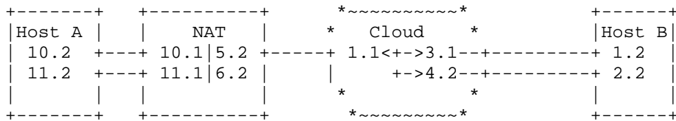
Fig 2: SCTP through NAT with multihoming
