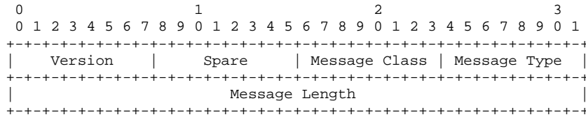
Figure 2 Common Message Header
