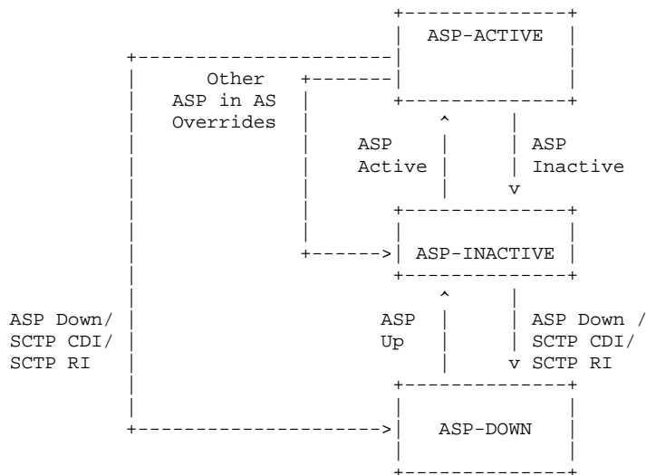
Figure 5: ASP State Transition Diagram
