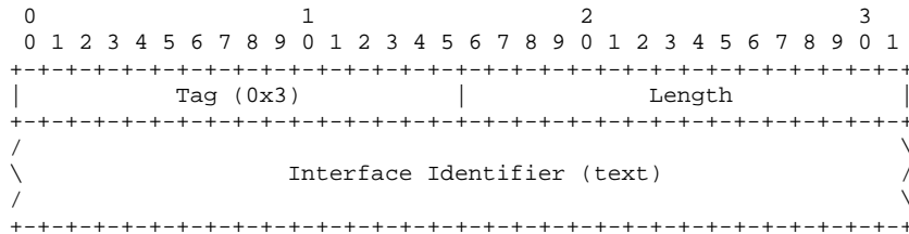
Figure 4 M2UA Message Header (Text-based Interface Identifier)
