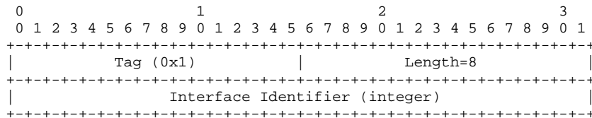
Figure 3 M2UA Message Header (Integer-based Interface Identifier)
