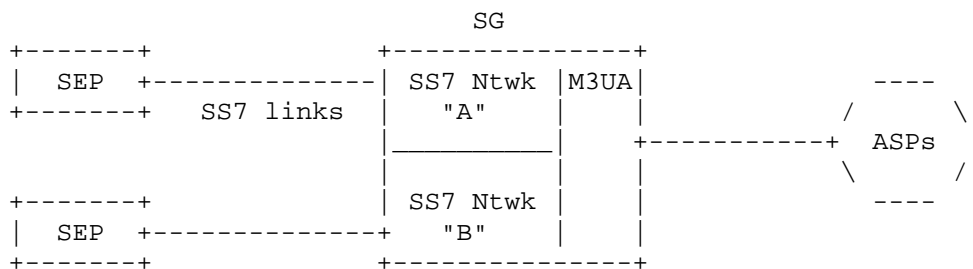
Figure 2 Example with multiple Network
