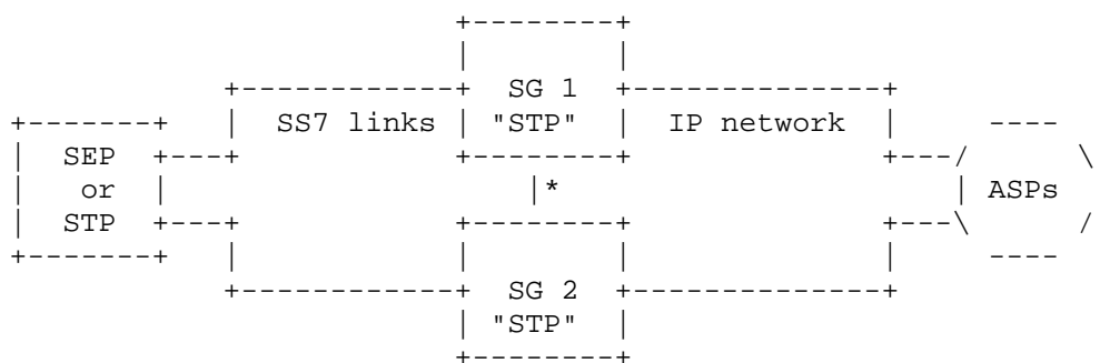
Figure 1 Example with mated SGs
