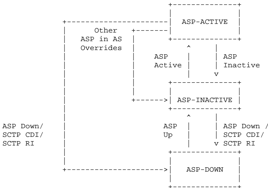
Figure 3: ASP State Transition Diagram, per AS
