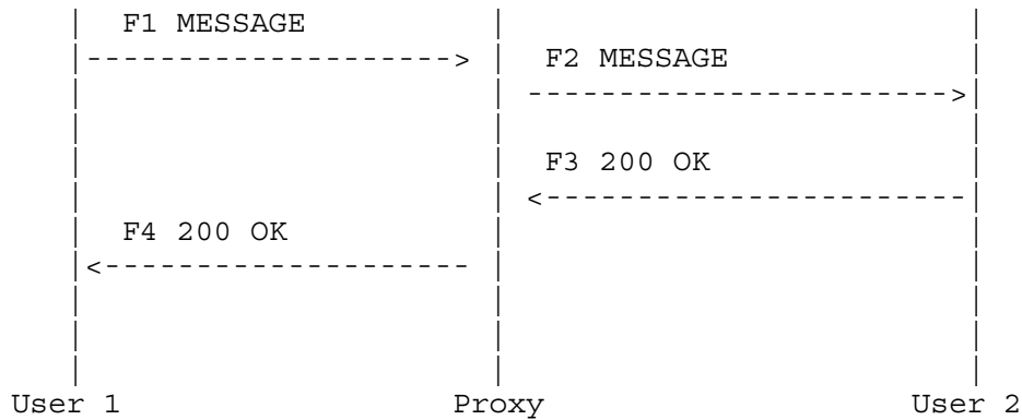
Figure 1: Example Message Flow
