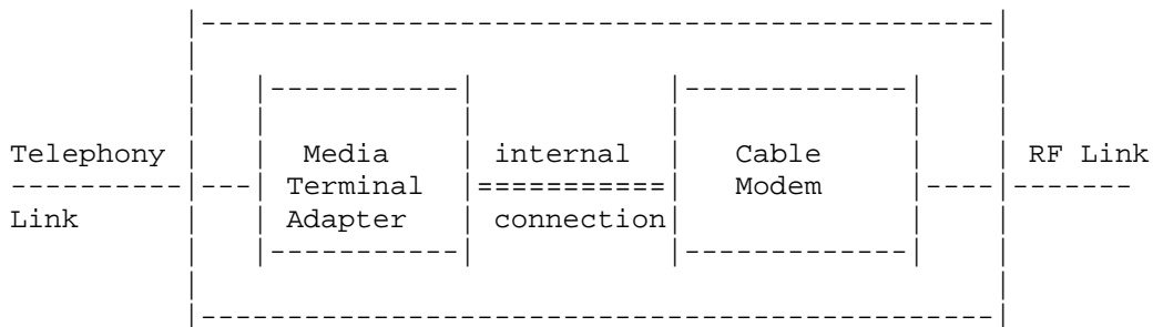
Figure 1. PacketCable 1.0 Embedded-MTA
