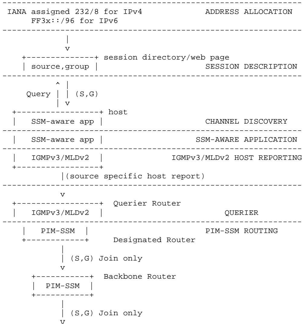
Figure 1: SSM Framework: elements in end-to-end model
