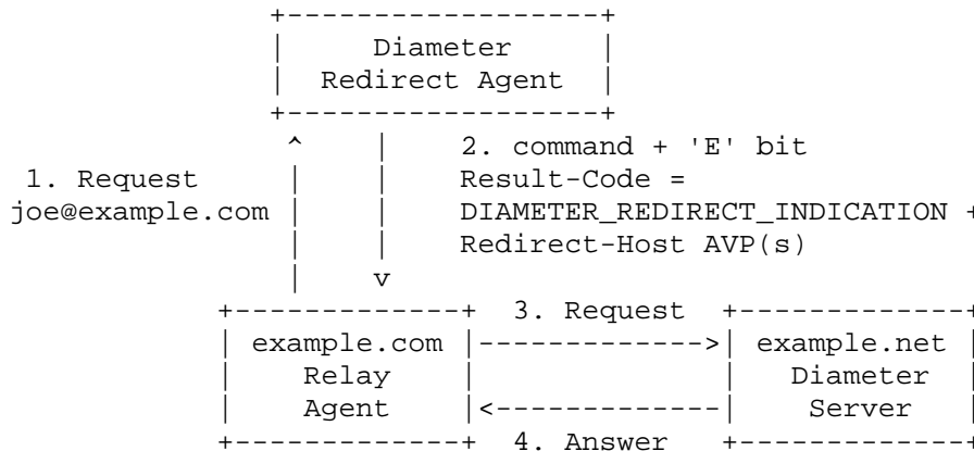
Figure 5: Diameter Redirect Agent
