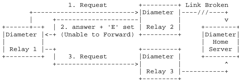
Figure 7: Example of Protocol Error causing answer message
