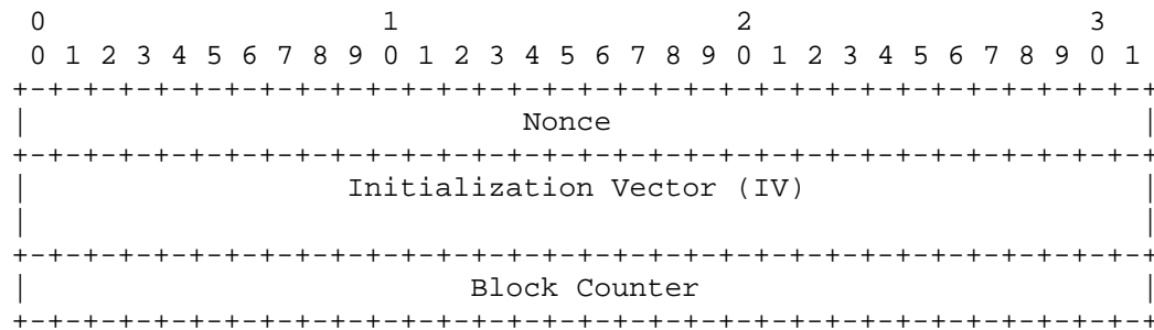
Figure 2. Counter Block Format
