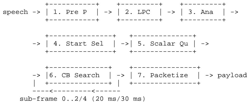
Figure 3.1. Flow chart of the iLBC encoder
