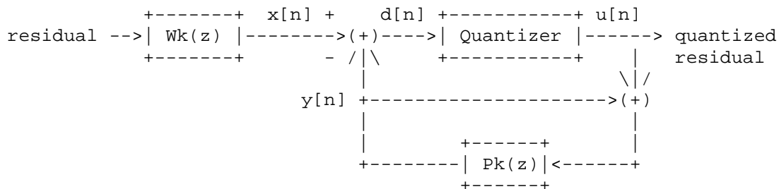
Figure 3.3. Quantization of start state samples by DPCM in weighted speech domain.
