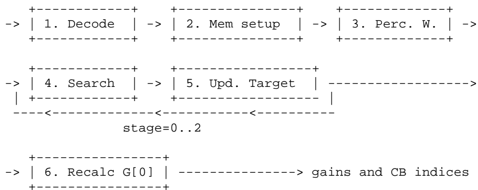
Figure 3.4. Flow chart of the codebook search in the iLBC encoder.
