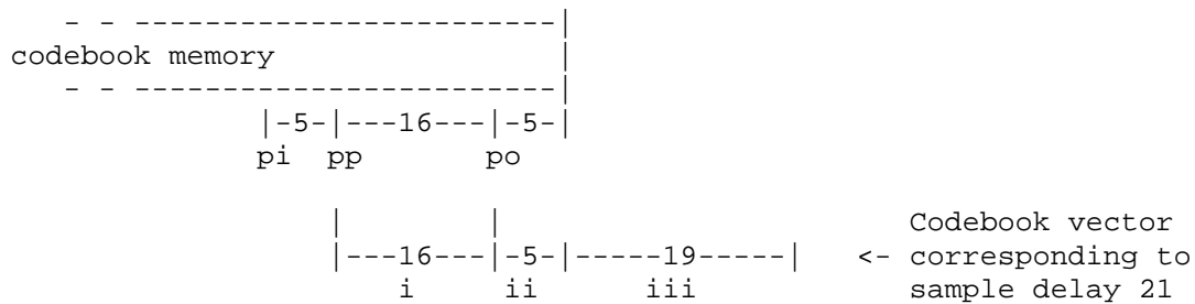
Figure 3.12. Generation of the second augmented codebook.
