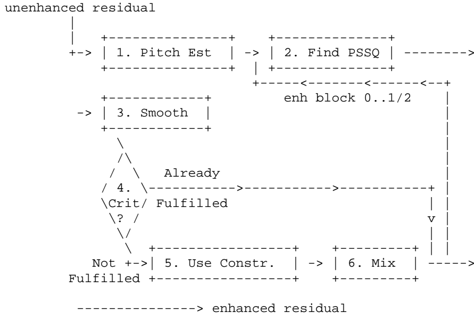
Figure 4.2. Flow chart of the enhancer.
