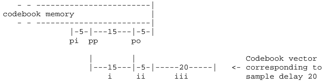
Figure 3.11. Generation of the first augmented codebook.
