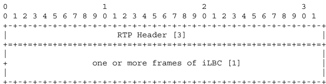
Figure 1, Packet format diagram
