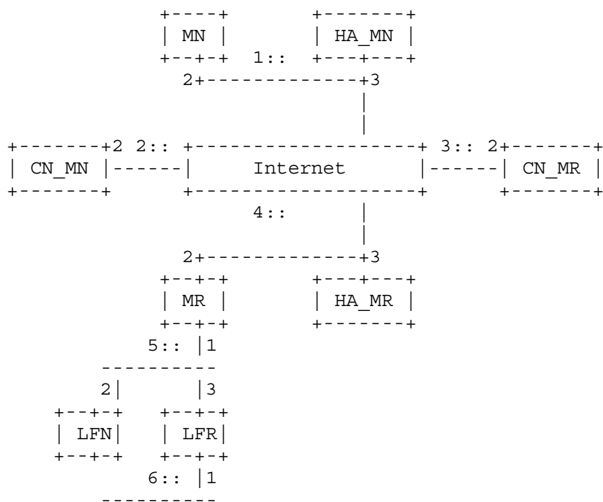
Figure 1. Mobile Router and Mobile Node at home.
