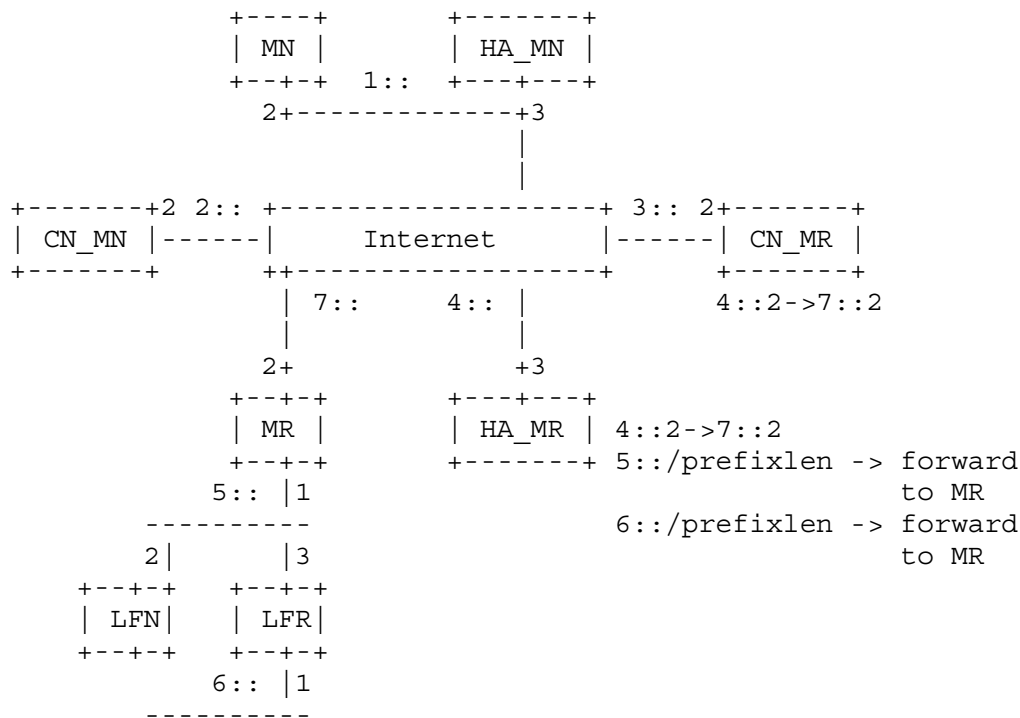
Figure 2. Mobile Router on a visited link.
