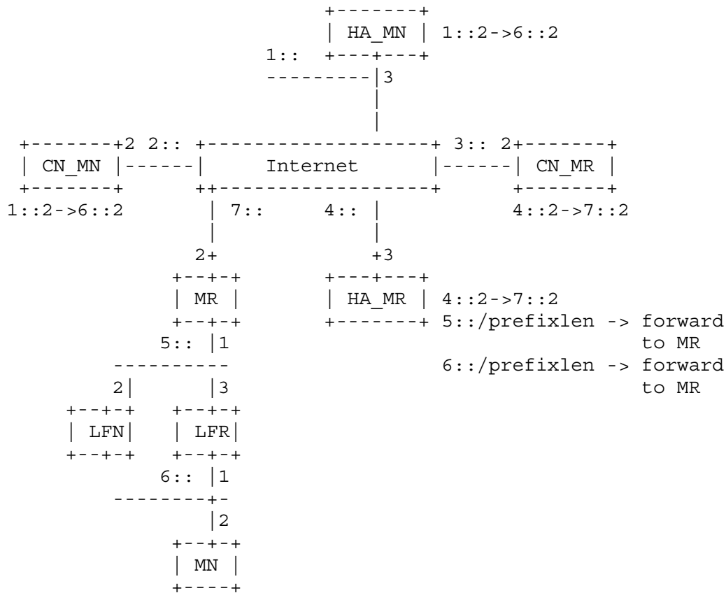
Figure 3. Mobile Node attached to Mobile Router on a visited link
