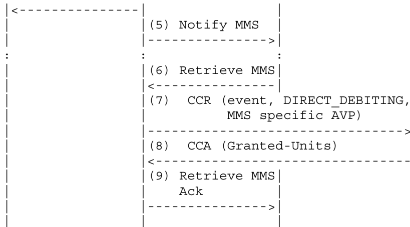
Figure A.4: Flow IV
