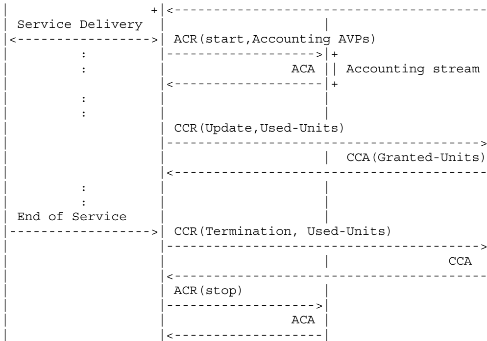
Figure 2: Protocol example with first interrogation after user's authorization/authentication
