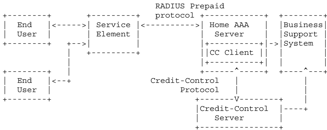
Figure 7: Credit-control architecture with service element containing translation agent, translating RADIUS prepaid to Diameter credit-control protocol
