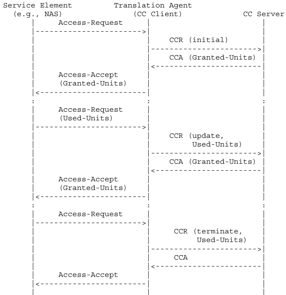
Figure 8: Message flow example with RADIUS prepaid - Diameter credit-control interworking
