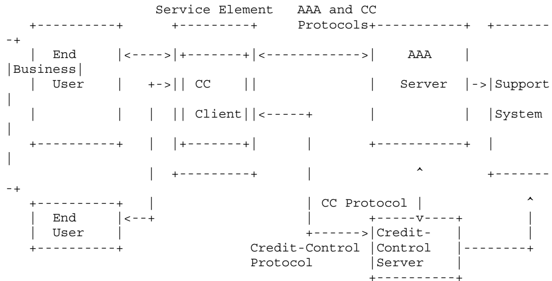
Figure 1: Typical credit-control architecture
