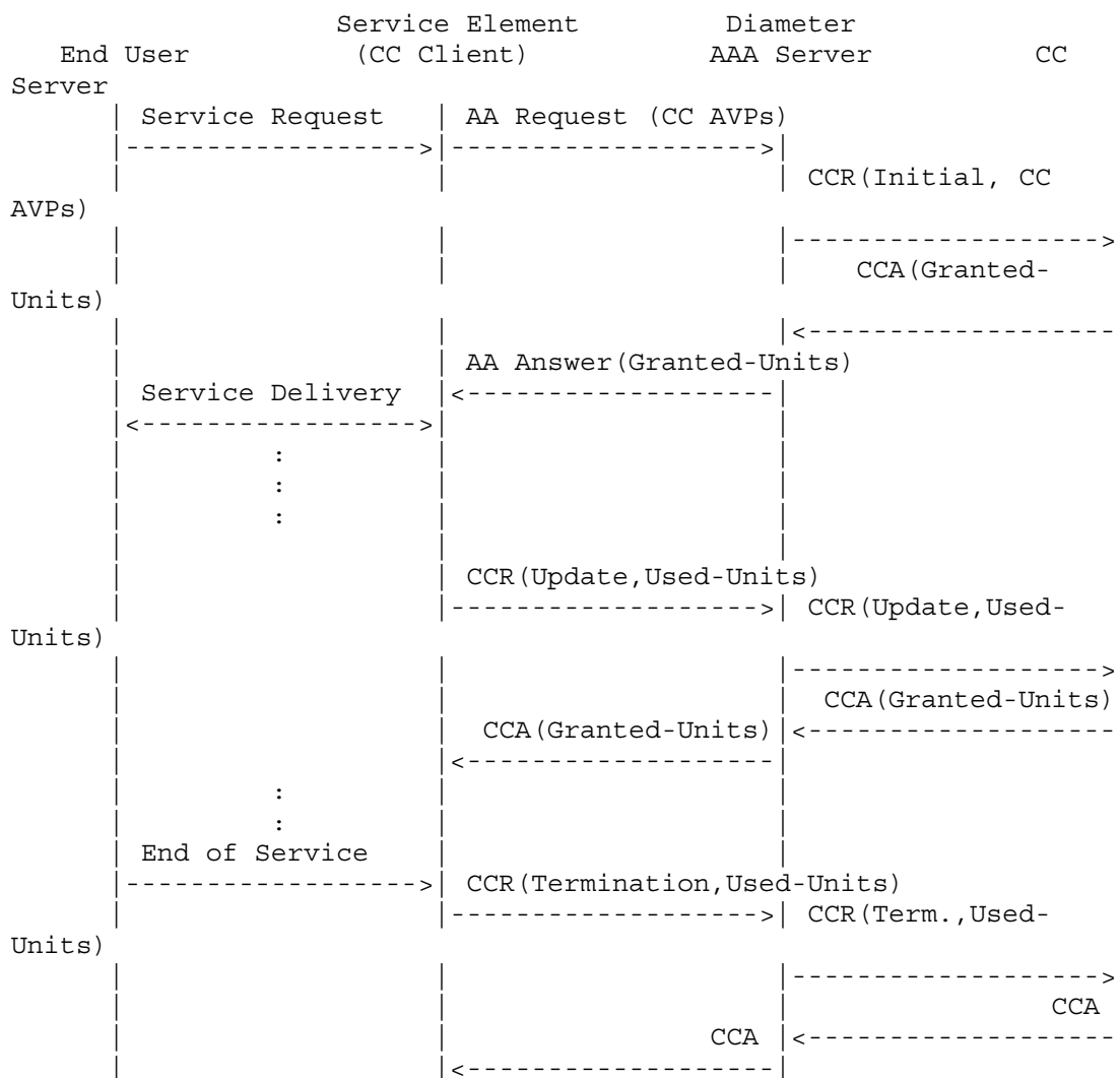
Figure 3: Protocol example with use of the authorization messages for the first interrogation
