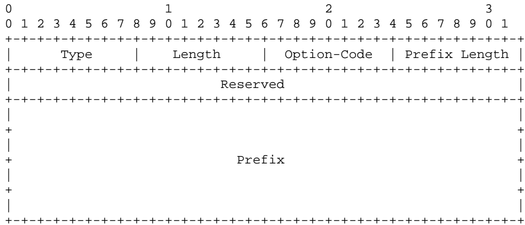
Figure 13: New Router Prefix Information Option
