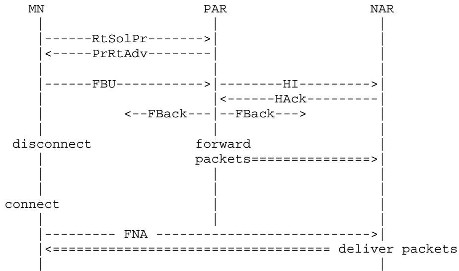
Figure 2: "Predictive" Fast Handover
