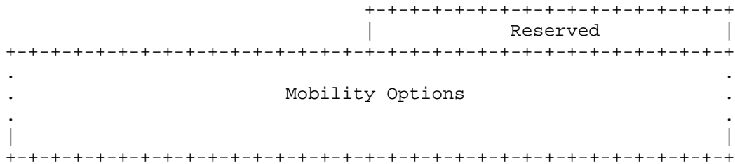
Figure 10: Fast Neighbor Advertisement (FNA) Message
