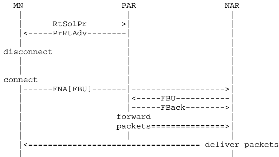
Figure 3: "Reactive" Fast Handover
