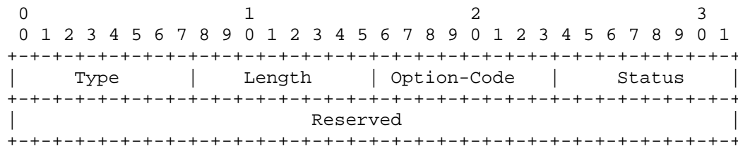
Figure 16: Neighbor Advertisement Acknowledgment Option
