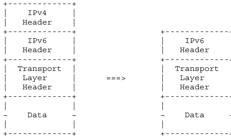
Decapsulating IPv6 from IPv4
