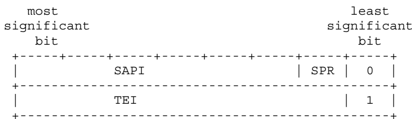
Figure 5. DLCI Format
