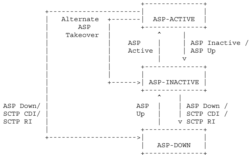
Figure 6. ASP State Transition Diagram
