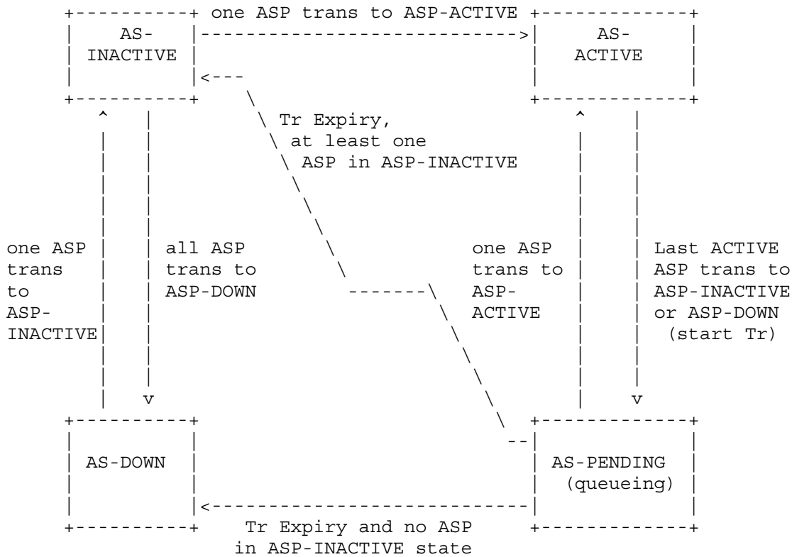
Figure 7: AS State Transition Diagram
