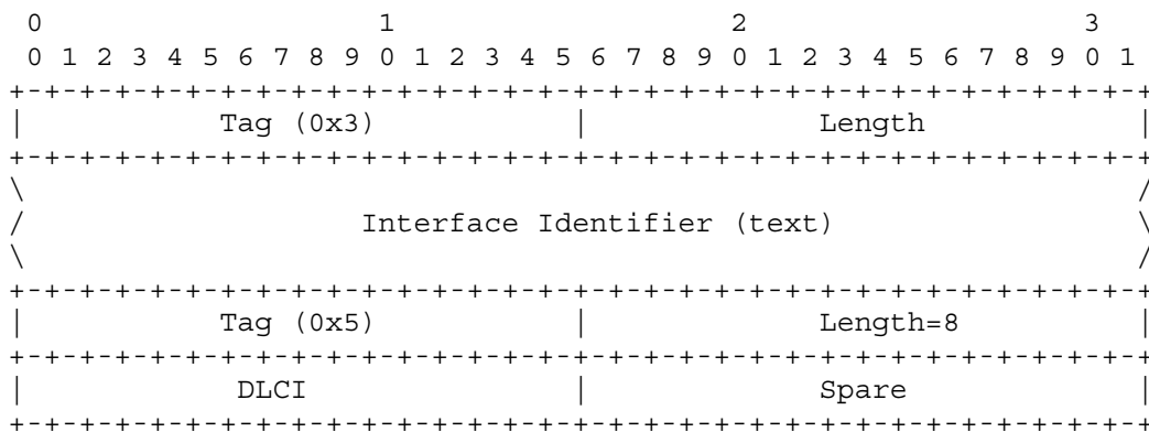
Figure 4. IUA Message Header (Text-based Interface Identifier)
