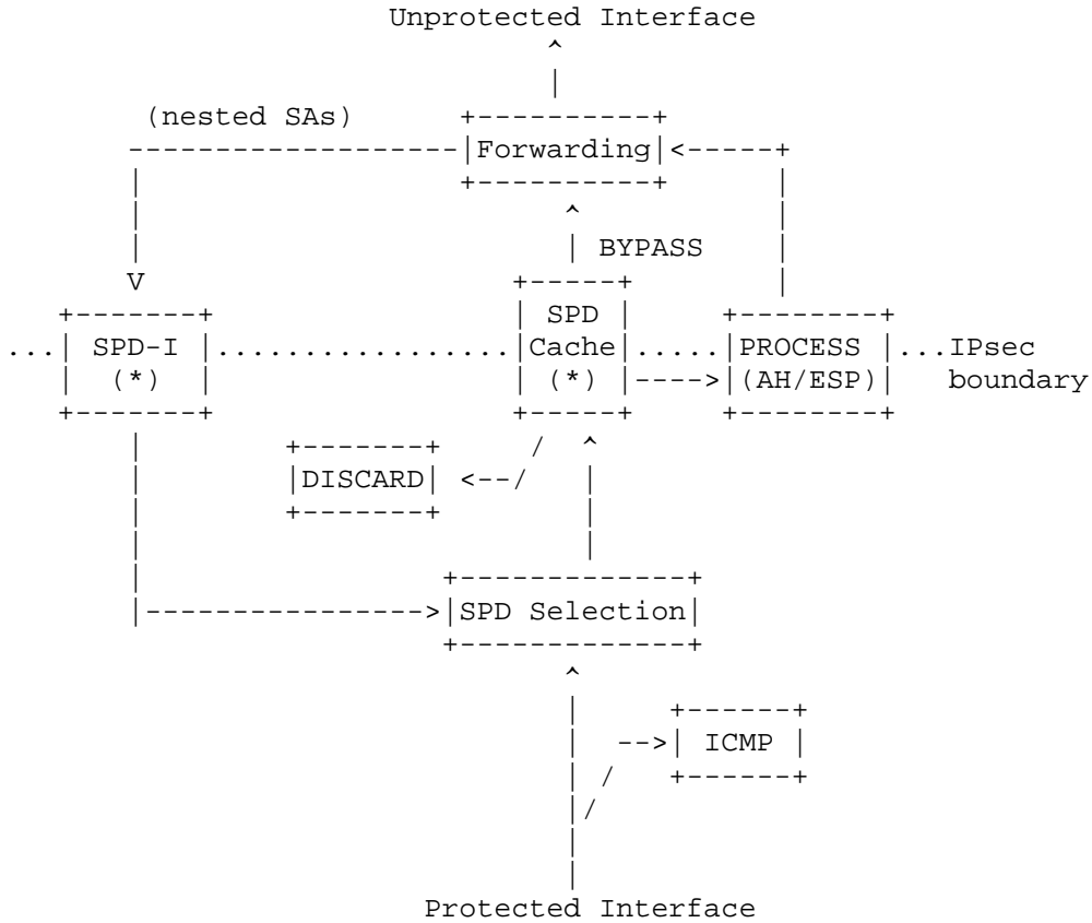
Figure 2. Processing Model for Outbound Traffic (*) = The SPD caches are shown here. If there is a cache miss, then the SPD is checked. There is no requirement that an implementation buffer the packet if there is a cache miss.
