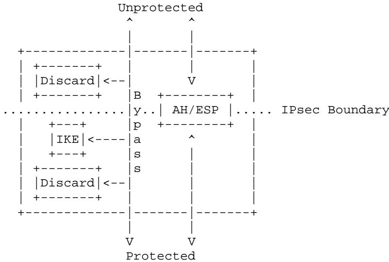
Figure 1. Top Level IPsec Processing Model
