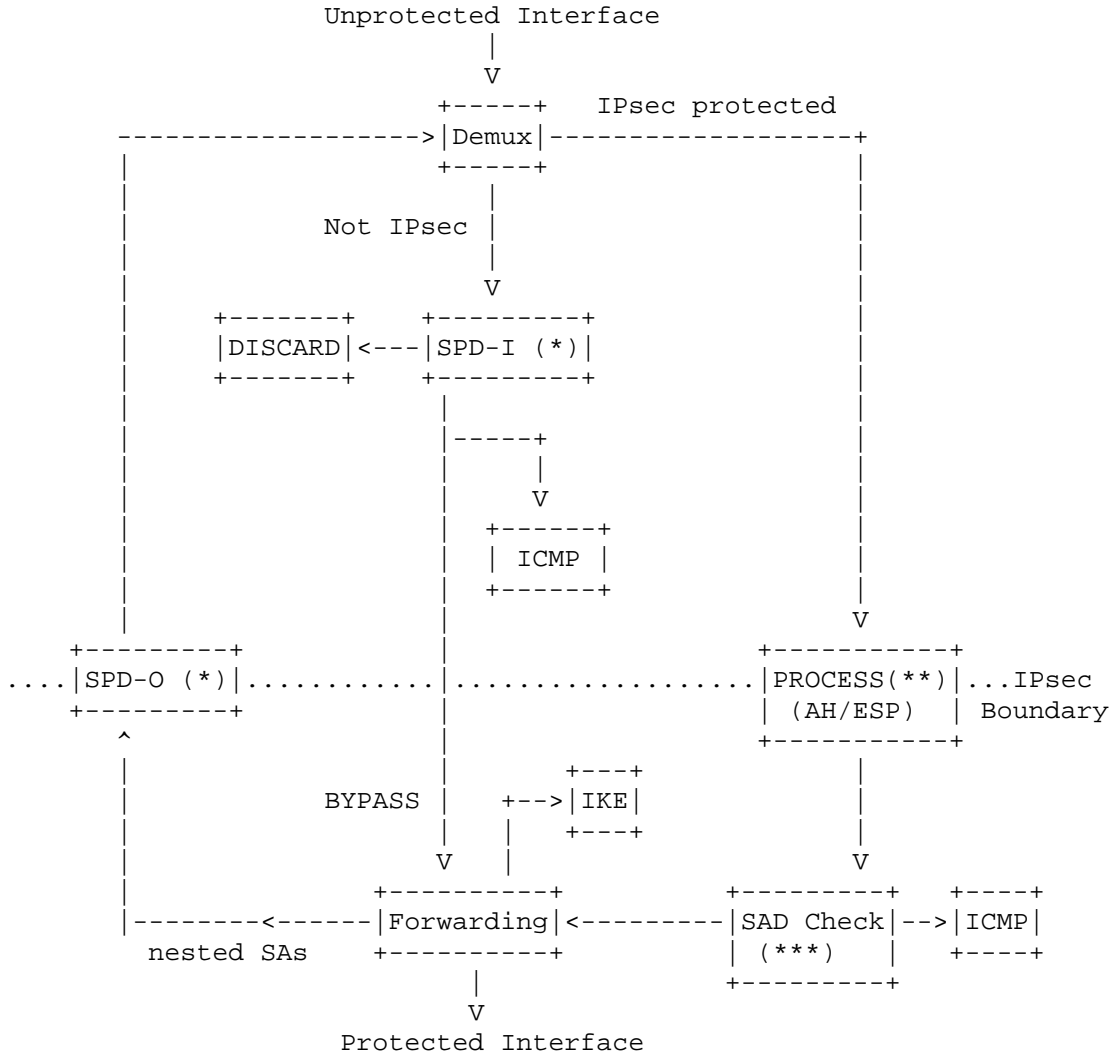
Figure 3. Processing Model for Inbound Traffic
