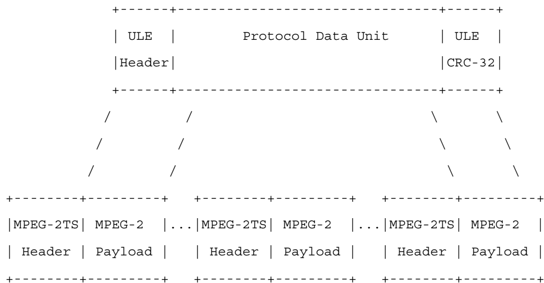
Figure 13: Encapsulation of an SNDU into a series of TS Packets
