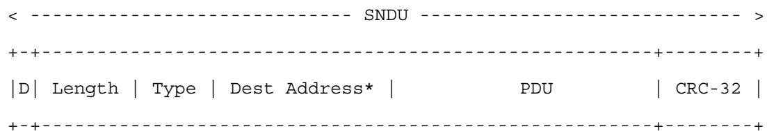
Figure 1: SNDU Encapsulation (* optional Destination Address)
