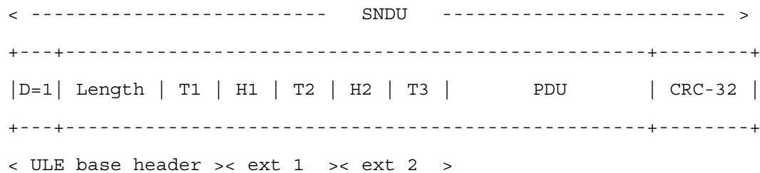
Figure 9: SNDU Encapsulation with two Extension Headers (D=1)
