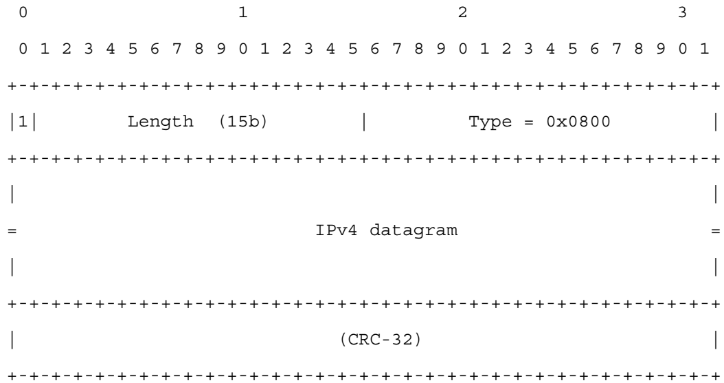
Figure 4: SNDU Format for an IPv4 Datagram using L3 filtering (D=1)
