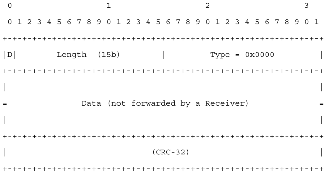
Figure 10: SNDU Format for a Test SNDU
