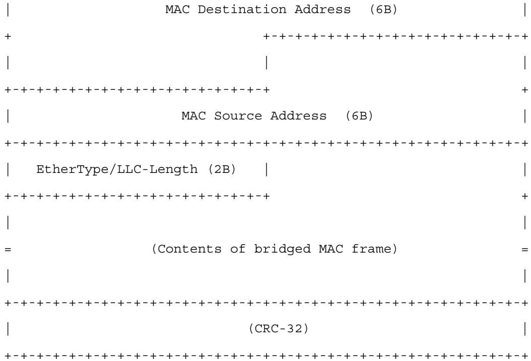
Figure 12: SNDU Format for a Bridged Payload (D=1)
