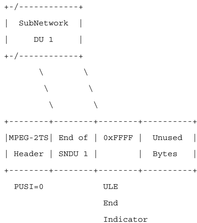
Figure 14: A TS Packet carrying the end of SNDU 1, followed by an
