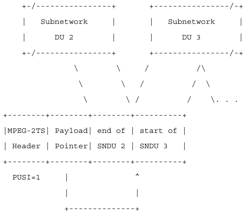
Figure 15: A TS Packet with the end of SNDU 2, followed by SNDU 3
