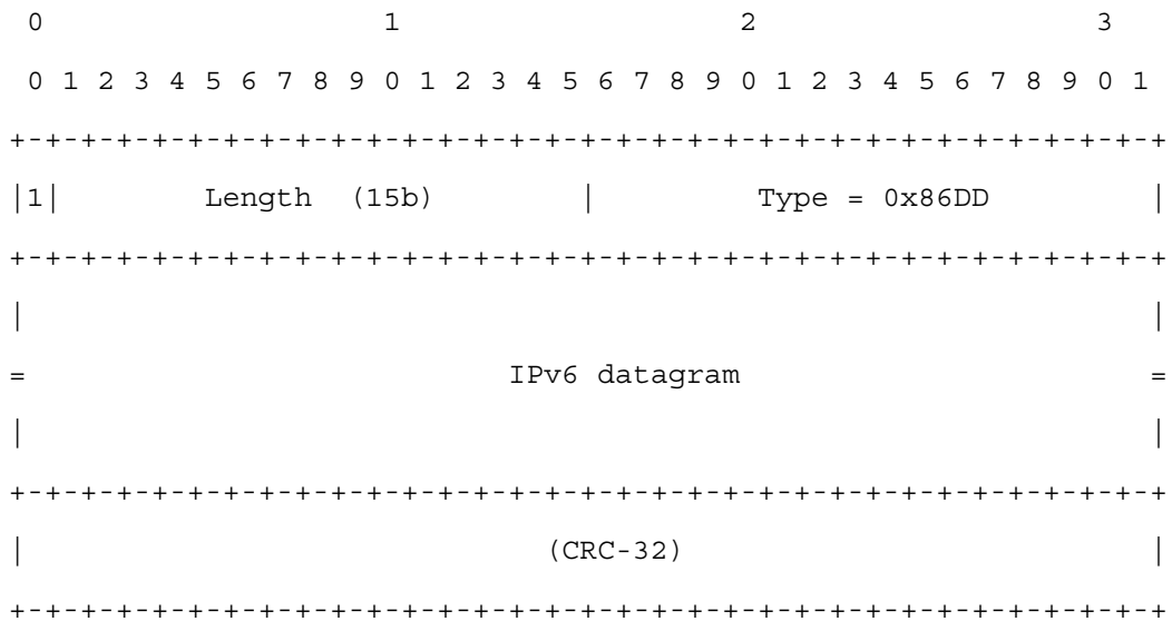
Figure 6: SNDU Format for an IPv6 Datagram using L3 filtering (D=1)
