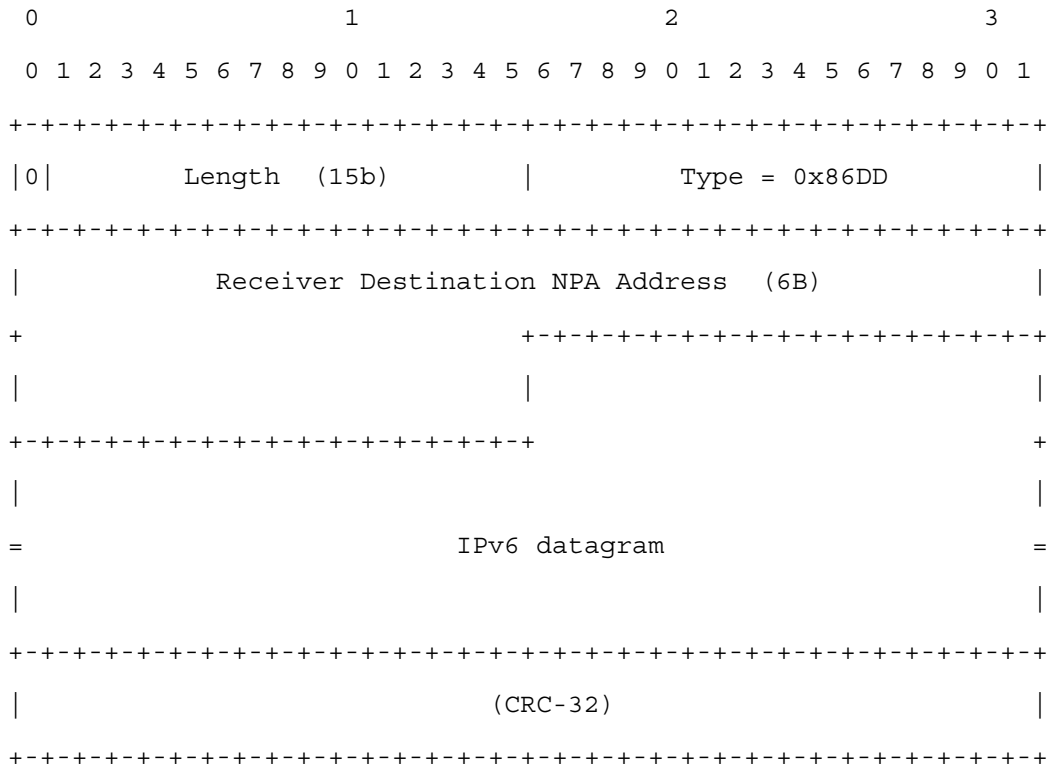
Figure 5: SNDU Format for an IPv6 Datagram using L2 filtering (D=0)
