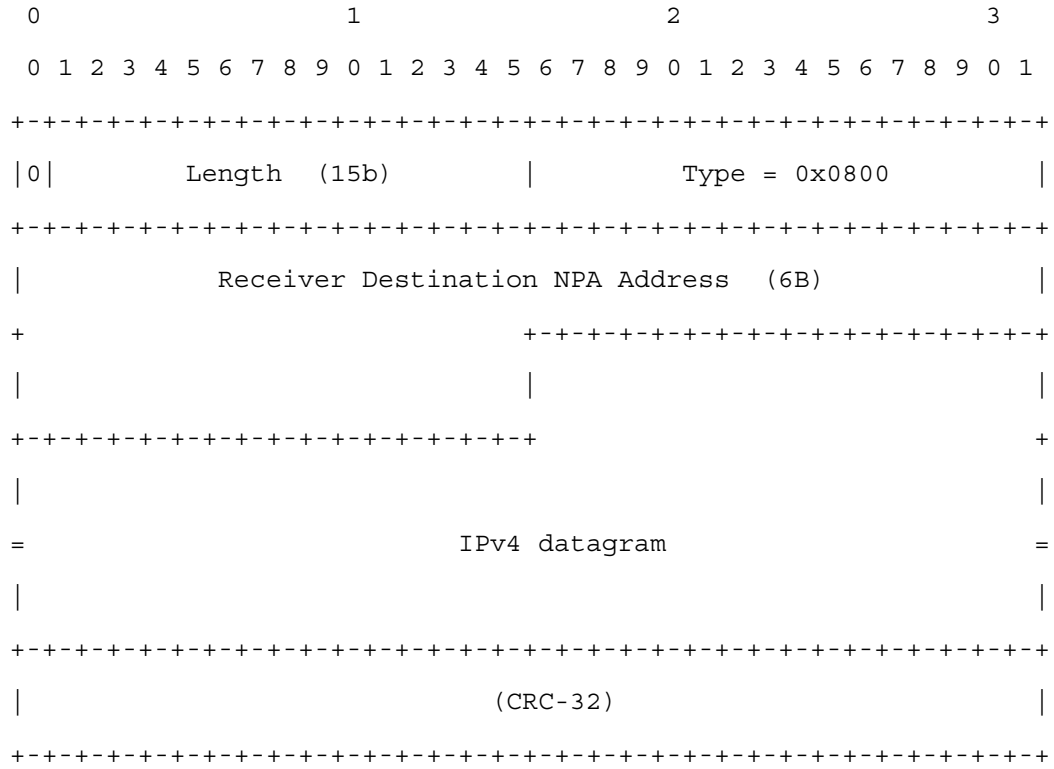
Figure 3: SNDU Format for an IPv4 Datagram using L2 filtering (D=0)
