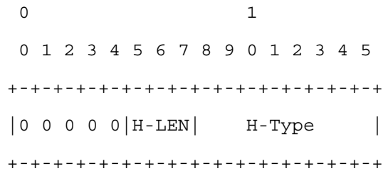
Figure 7: Structure of ULE Next-Header Field
