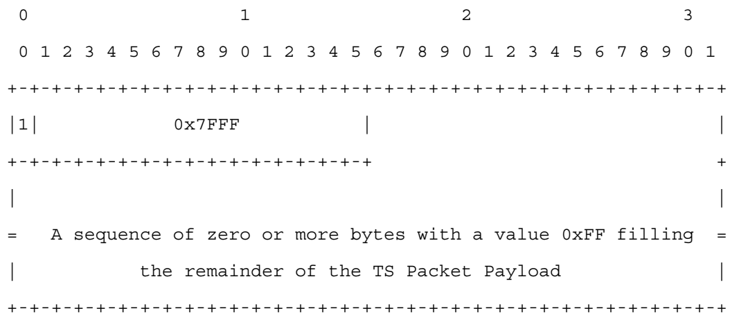
Figure 2: Format for a ULE End Indicator
