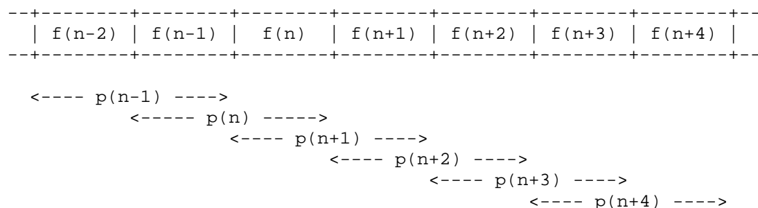
Figure 1: An example of redundant transmission
