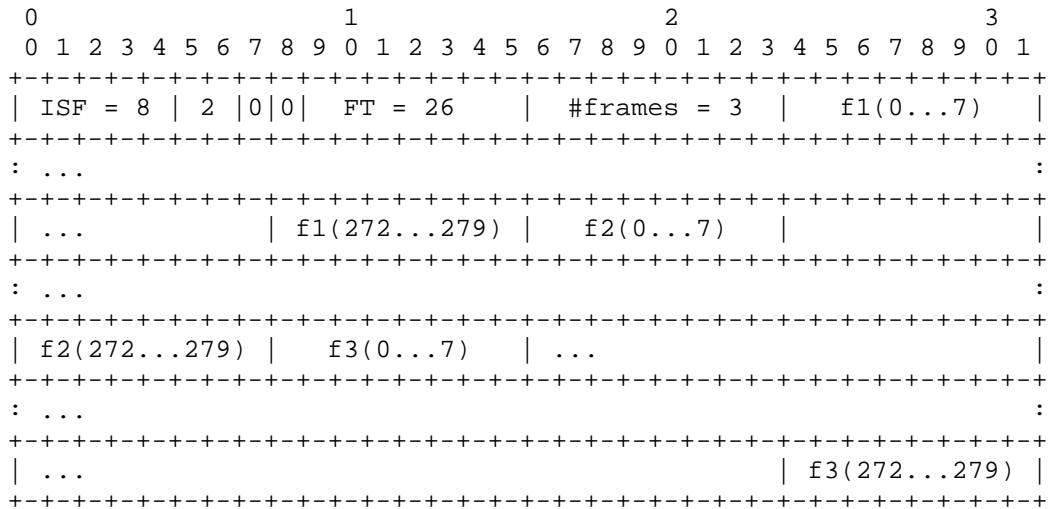
Figure 4: An example of a basic mode payload carrying three frames of the same frame type
