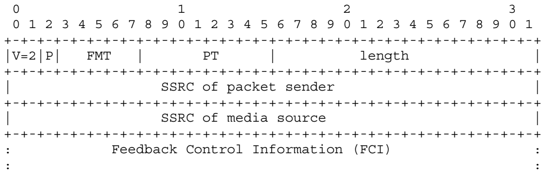
Figure 3: Common Packet Format for Feedback Messages
