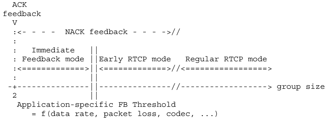
Figure 1: Modes of operation
