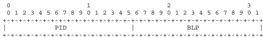
Figure 4: Syntax for the Generic NACK message
