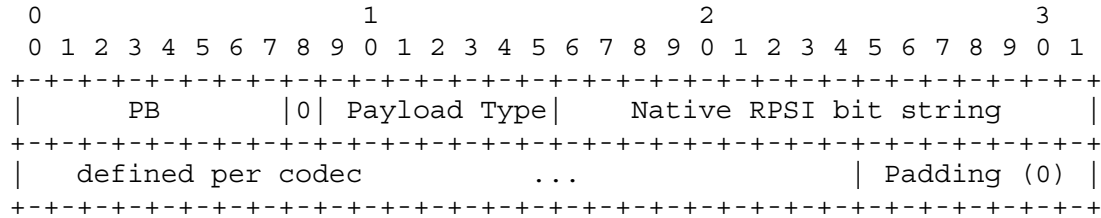
Figure 7: Syntax of the Reference Picture Selection Indication (RPSI)
