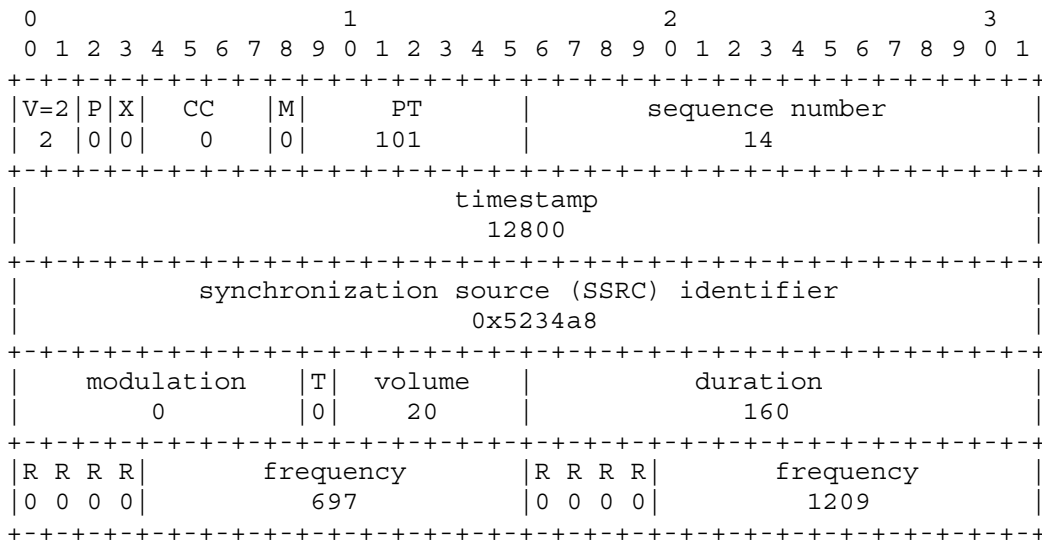
Figure 4: Example RTP Packet for Tone Payload
