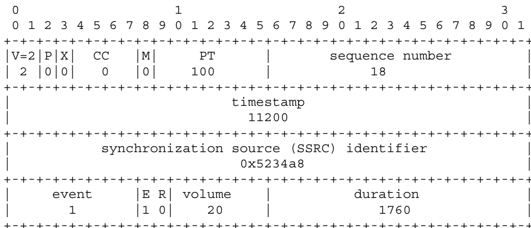
Figure 3: Example RTP Packet for Event Payload
