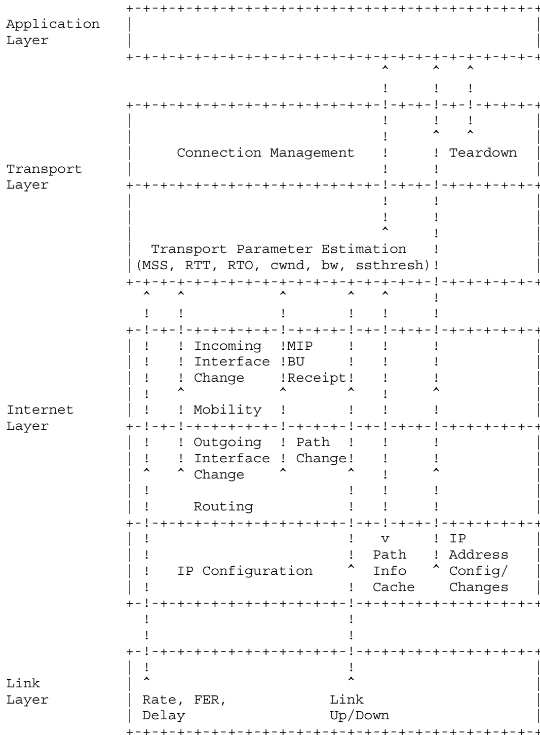
Figure 1. Layered Indication Model
