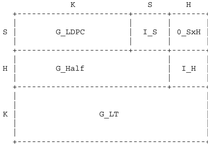
Figure 4: The matrix A
