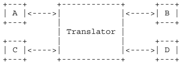
Figure 4 - RTP Translator (Relay) with Only Unicast Paths
