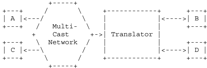
Figure 3 - Point to Multipoint Using a Translator
