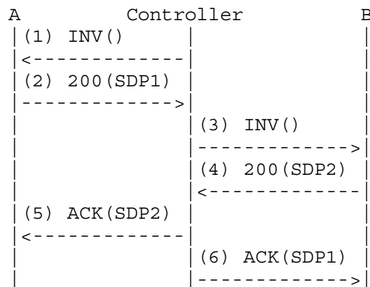
Figure 12: Role Conflict Flow
