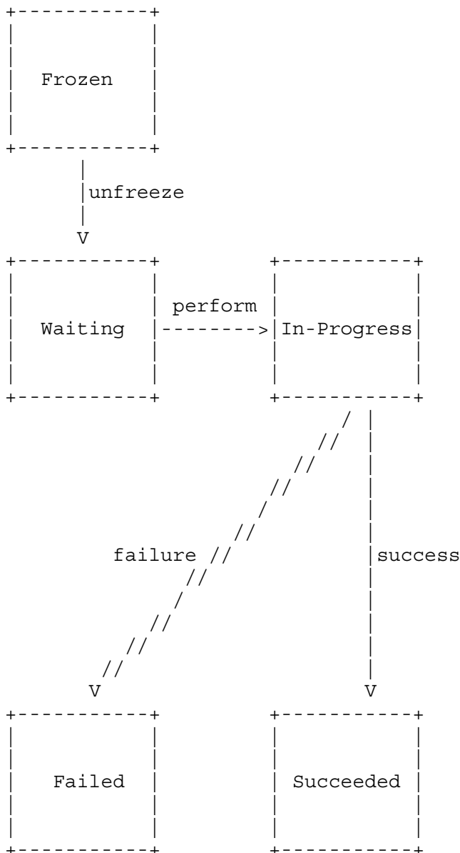
Figure 7: Pair State FSM
