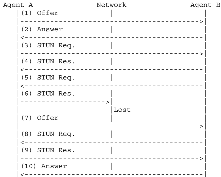
Figure 11: Race Condition Flow
