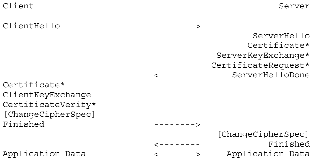
Figure 1. Message flow for a full handshake
