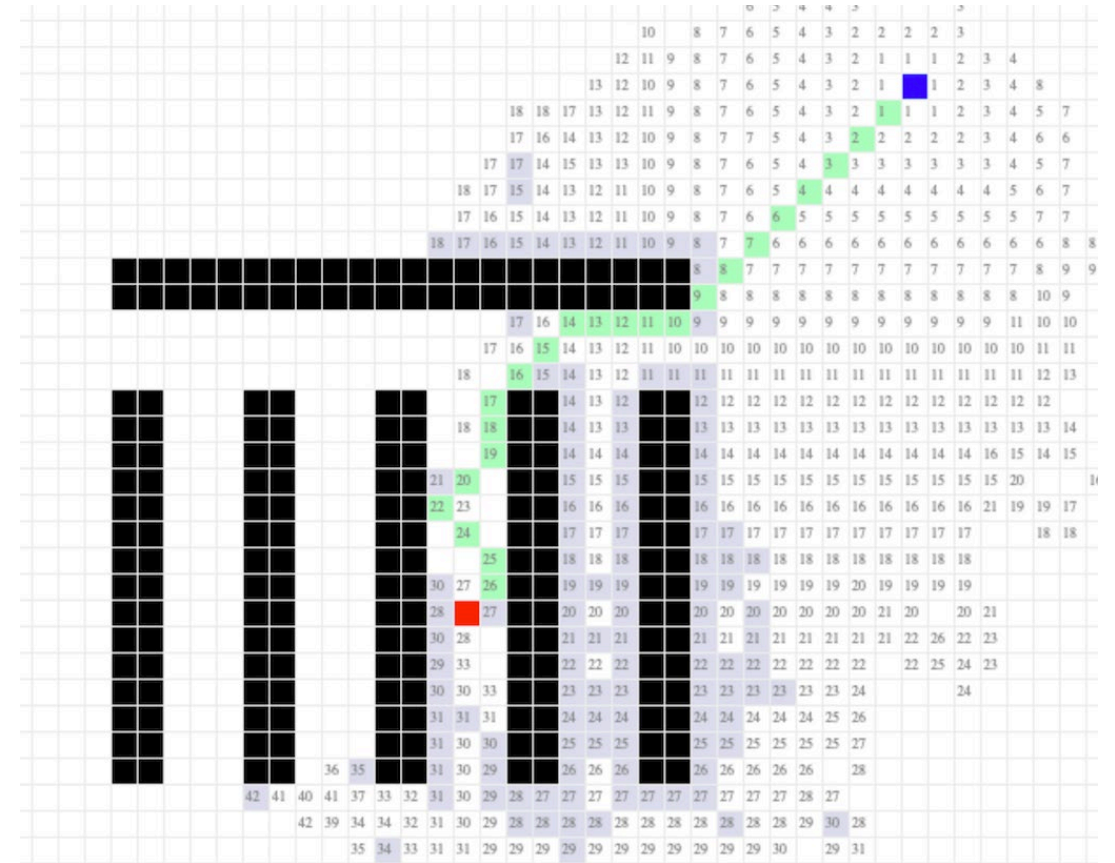
Ant Swarm
