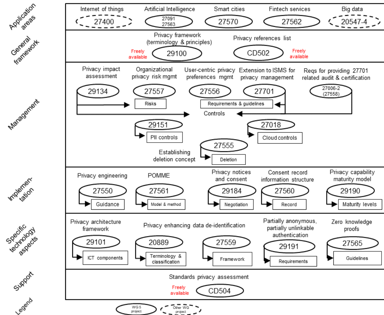
Figure 1: Overview of privacy/PII publications and projects in SC 27, mainly WG 5
