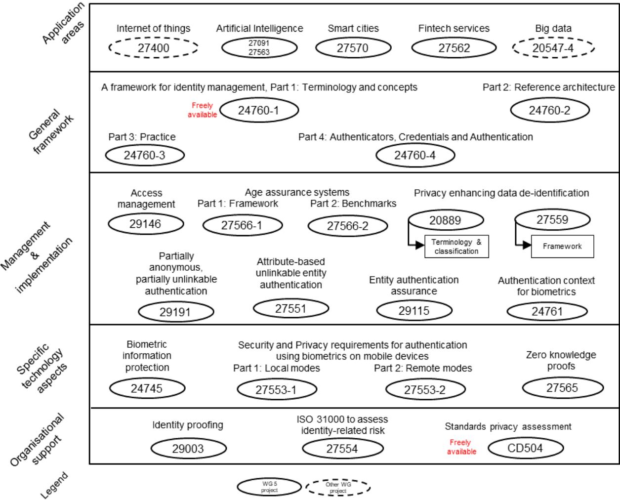
Figure 2: Overview of identity management publications and projects in SC 27, mainly WG 5
