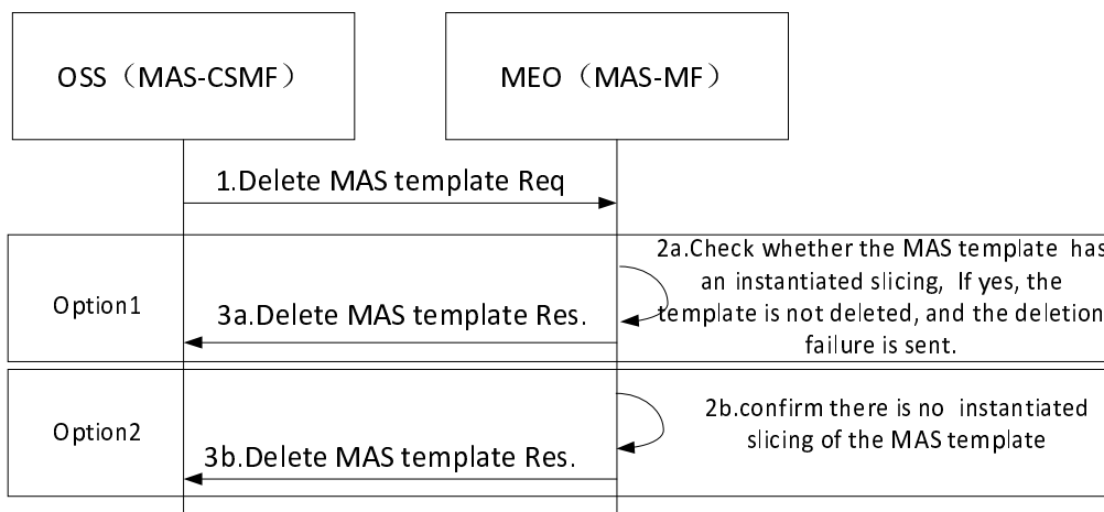
Figure 6.4.7-1: Delate MEC Application Slice Template
