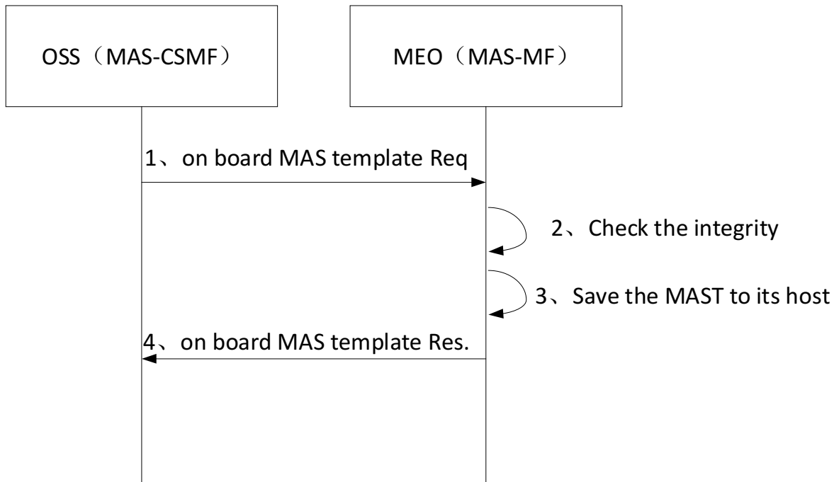
Figure 6.4.2-1: On-board MEC Application Slice Template
