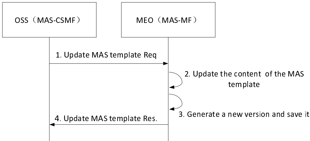
Figure 6.4.6-1: Update MEC Application Slice Template
