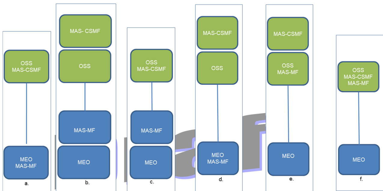
Figure 6.2.2-1: Possible combinations of newly introduced entities and MEC system
