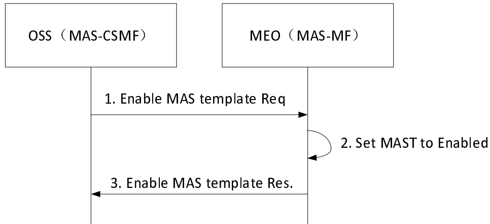
Figure 6.4.4-1: Enable MEC Application Slice template
