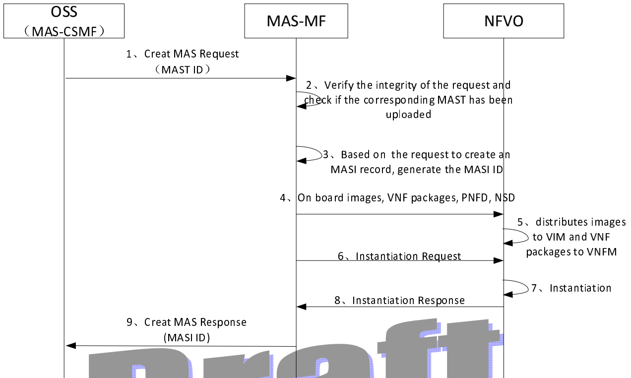
Figure 6.5.3-1: Creating a MAS process
