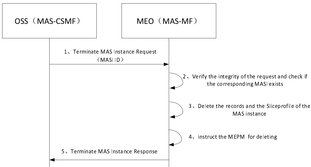
Figure 6.5.5-1: Terminate a MASI
