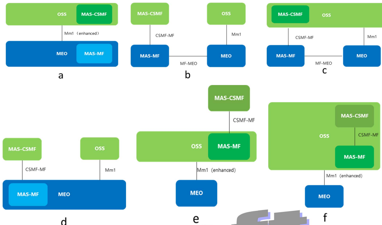
Figure 6.3.2-1: Detailed analysis of each combination based on interface
