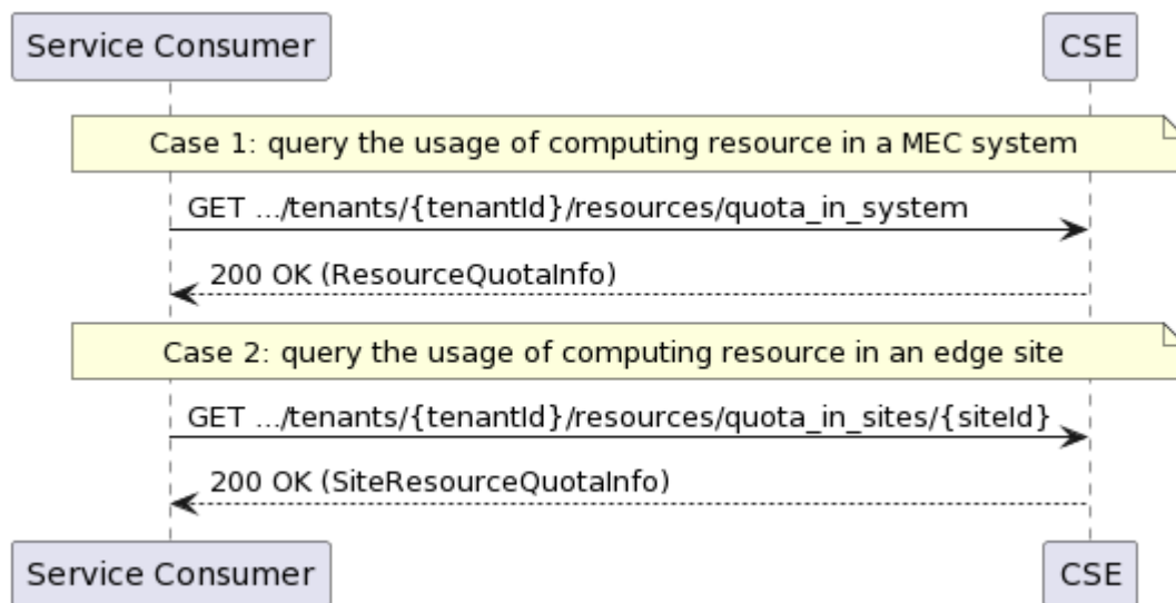
Figure 5.2.3.4-1: Flow of querying the computing resource quota
