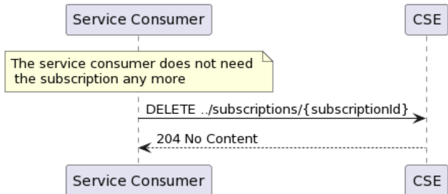
Figure 5.2.4.4-1: Flow of unsubscribing from the CSE event notifications
