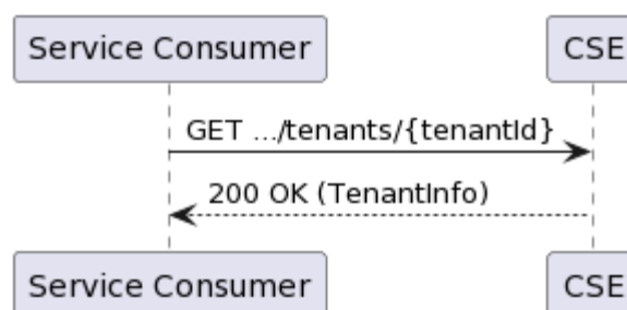
Figure 5.2.2.5-1: Flow of querying a specific tenant resource
