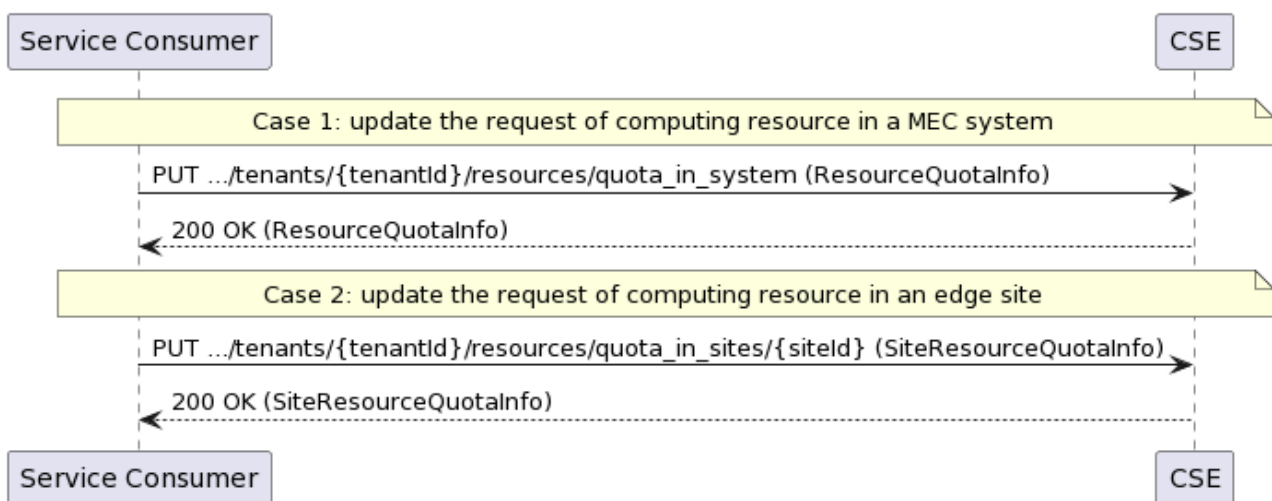
Figure 5.2.3.3-1: Flow of updating the computing resource request
