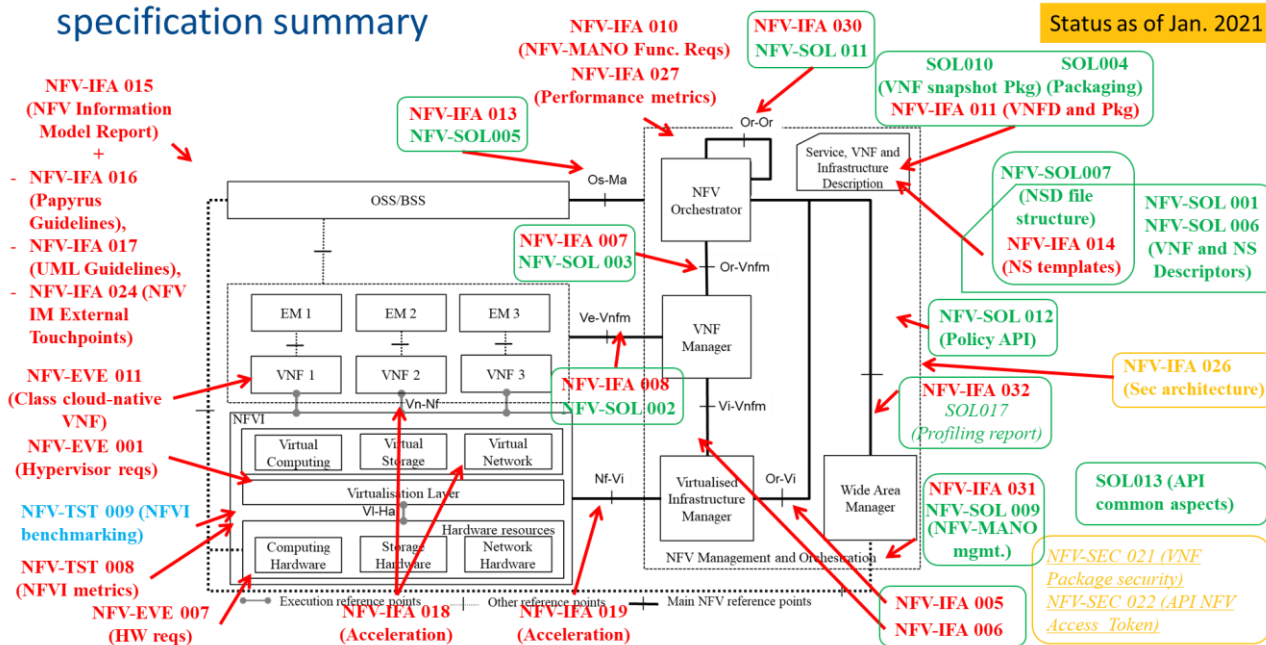
Figure 6.7-1: Map of ETSI NFV specifications, reports, and the NFV Architectural Framework.
